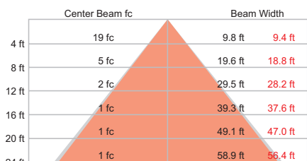
17.5 ft (5.3 m) 1 fc maximum distance ■ Vert. Spread: 101.7° ■ Horiz. Spread: 99.2°
