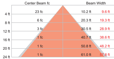
19.4 ft (5.9 m) 1 fc maximum distance ■ Vert. Spread: 103.6° ■ Horiz. Spread: 100.6°
