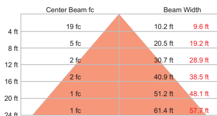
17.3 ft (5.3 m) 1 fc maximum distance ■ Vert. Spread: 104.0° ■ Horiz. Spread: 100.5°
