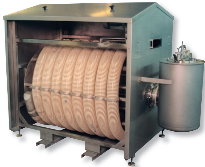
4" spiralpumpe for pumpning af muslinger
