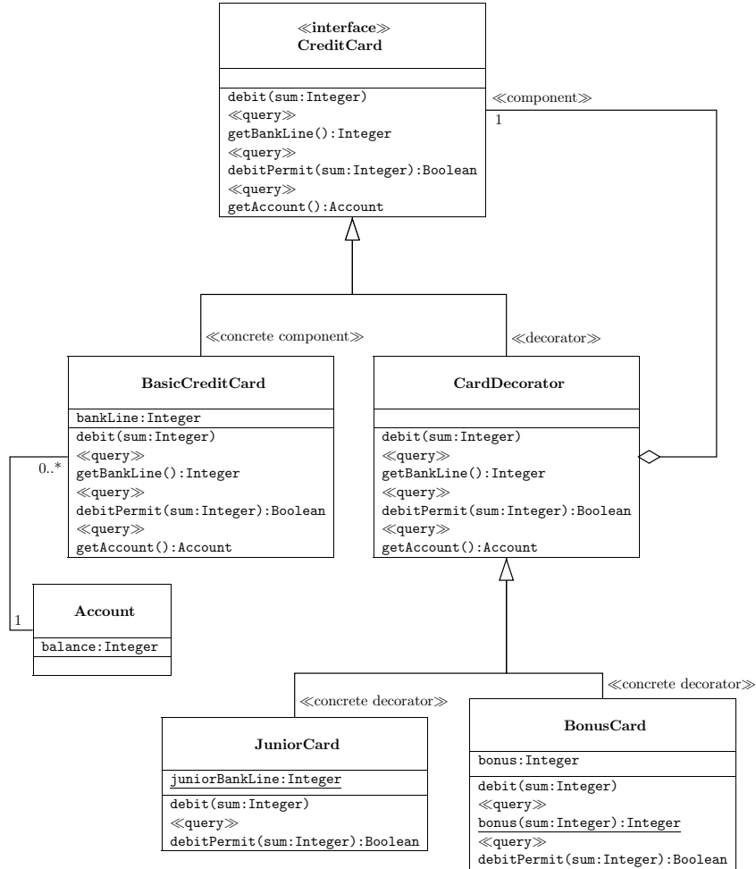
Fig. 6 Credit card diagram with Decorator pattern
