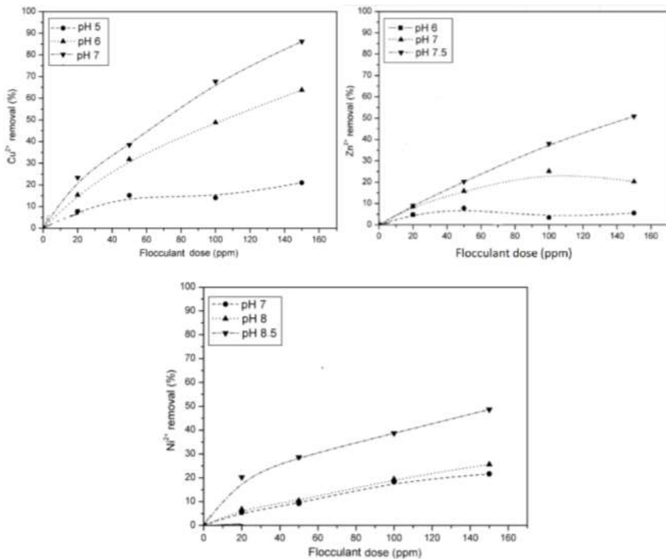
Figure 7. Removal of \text{Cu}^{2+} , \text{Zn}^{2+} , and \text{Ni}^{2+} ions from water depending on the dosage of the flocculant and the pH of the water
