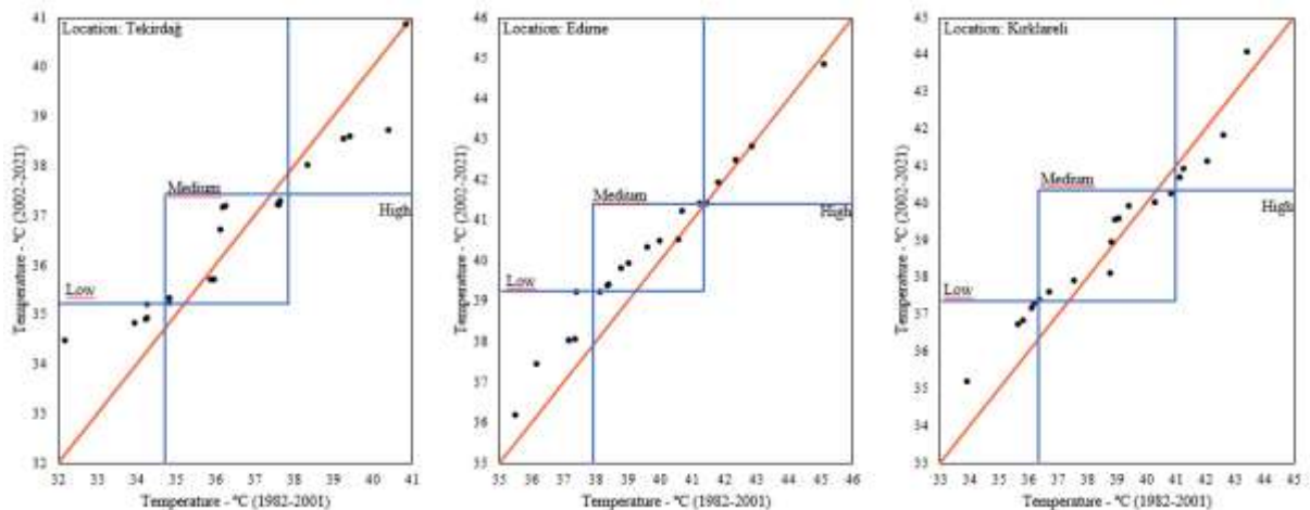
Figure 6. Maximum temperature at 2 meters
