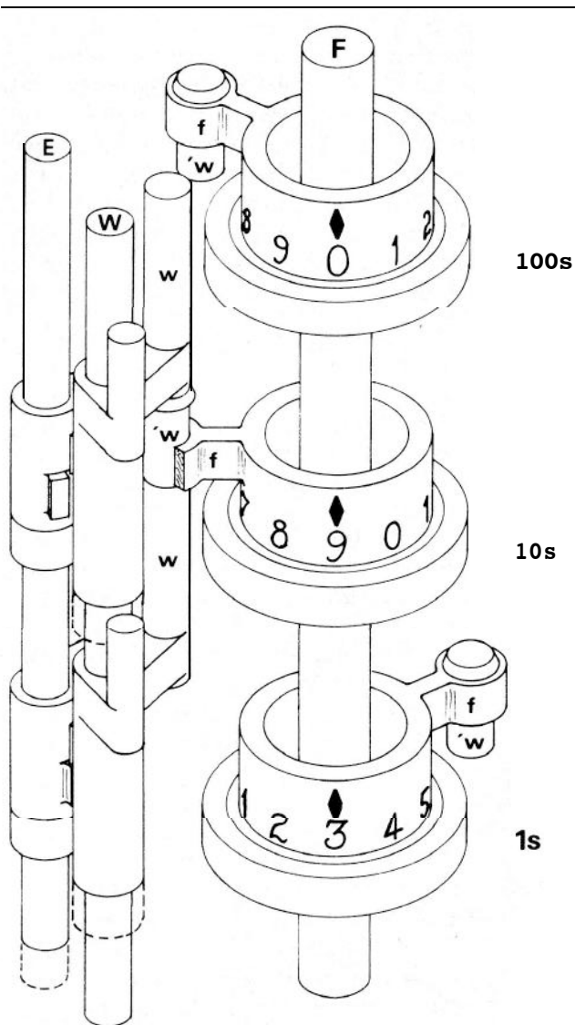
Figure 7. “Anticipating carry.” The movable wire ‘w’ carried in the arm of the figure wheel may interpose between the fixed wires w to propagate a carry through several cages. In the figure a carry is generated in the units cage. Because the tens figure wheel stands at 9, a carry is propagated to the hundreds cage. The hundreds figure wheel does not stand at 9 and therefore breaks the chain of carry propagation.
