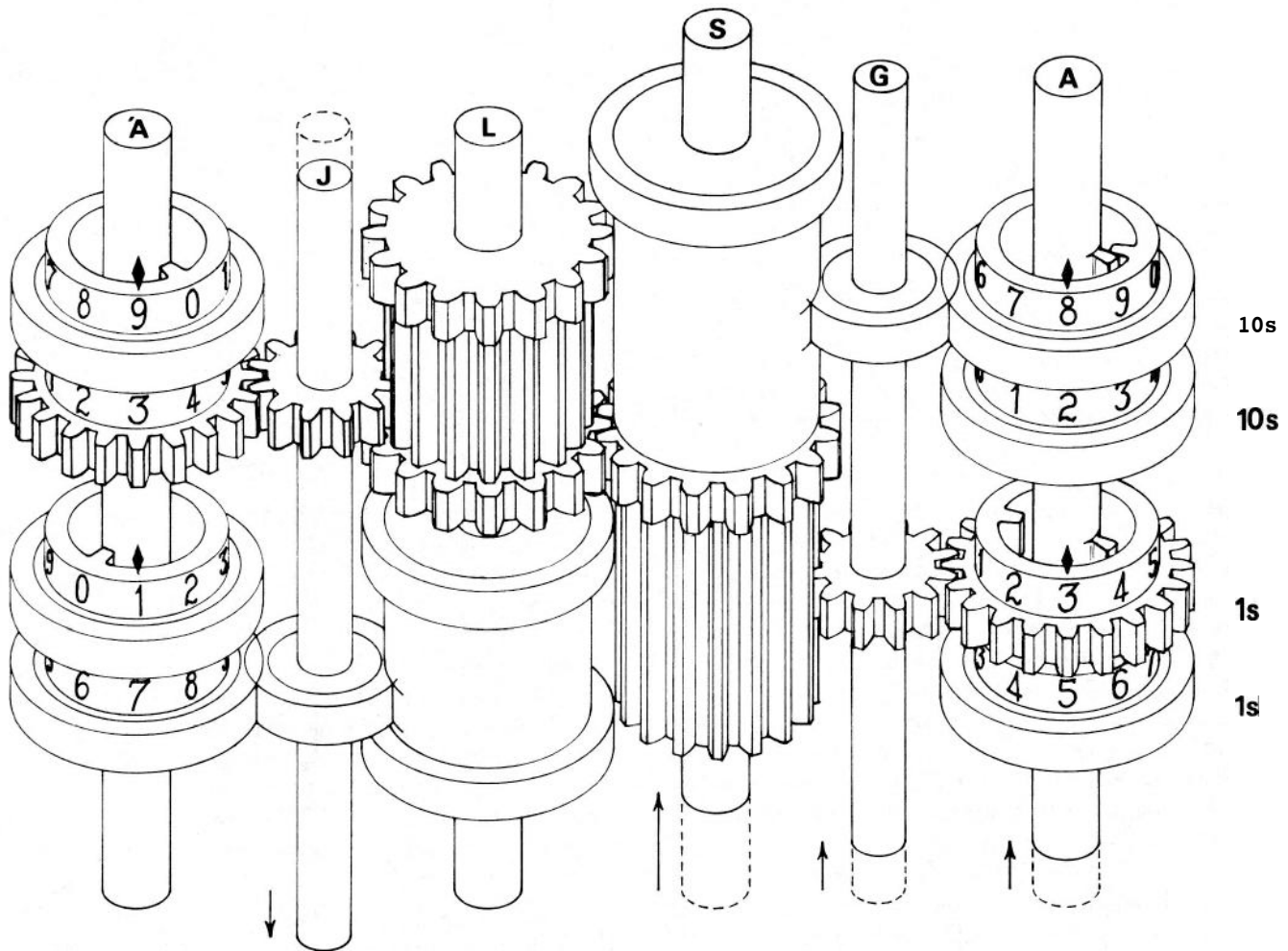
Figure 4. Process of stepping, or multiplication, and division by 10. The “ long pinions ” S are raised with their axis to engage the long pinions L in the cage above. A number given off will therefore be stepped up a cage, or multiplied by 10. A transfer in the reverse direction will divide by 10.
