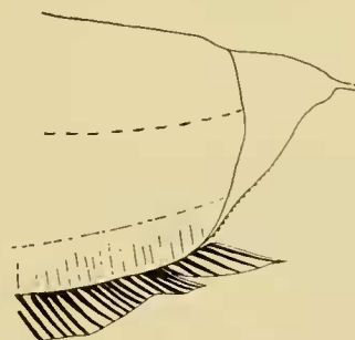
FIG. 19. Regenerated Tail. Gymnotus carapo (Linnæus), Rio Coite.
