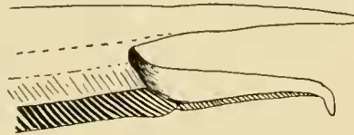
FIG. 21. Split Tail. Gymnotus carapo (Linnæus), Aqua Quente, Paraguay.
