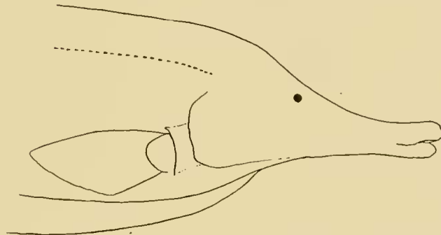
FIG. 10. Sternarchorhamphus mülleri (Steindachner).
