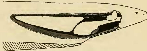
FIG. 29. Section showing location of air-bladder in Gymnotus carapo Linnæus.
