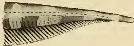
FIG. 22. Normal Tail. Gymnotus carapo (Linnæus), Holmia, British Guiana.
