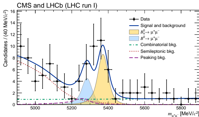
Figure 1.9: Dimuon invariant mass of B candidates showing peaks corresponding B_s^0 \rightarrow \mu^+ \mu^- and B^0 \rightarrow \mu^+ \mu^- decays [44].
