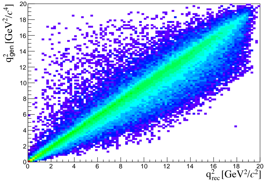
Figure 5.26: Generated versus reconstructed q^2 for simulated B^0 \rightarrow K^{*0}e^+e^- events.
