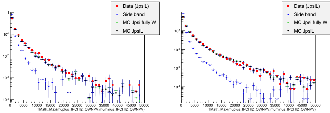
Figure A.2: Distributions of maximum muon IP\chi^2 variable in data and simulation for LL (left) and DD (right) events.
