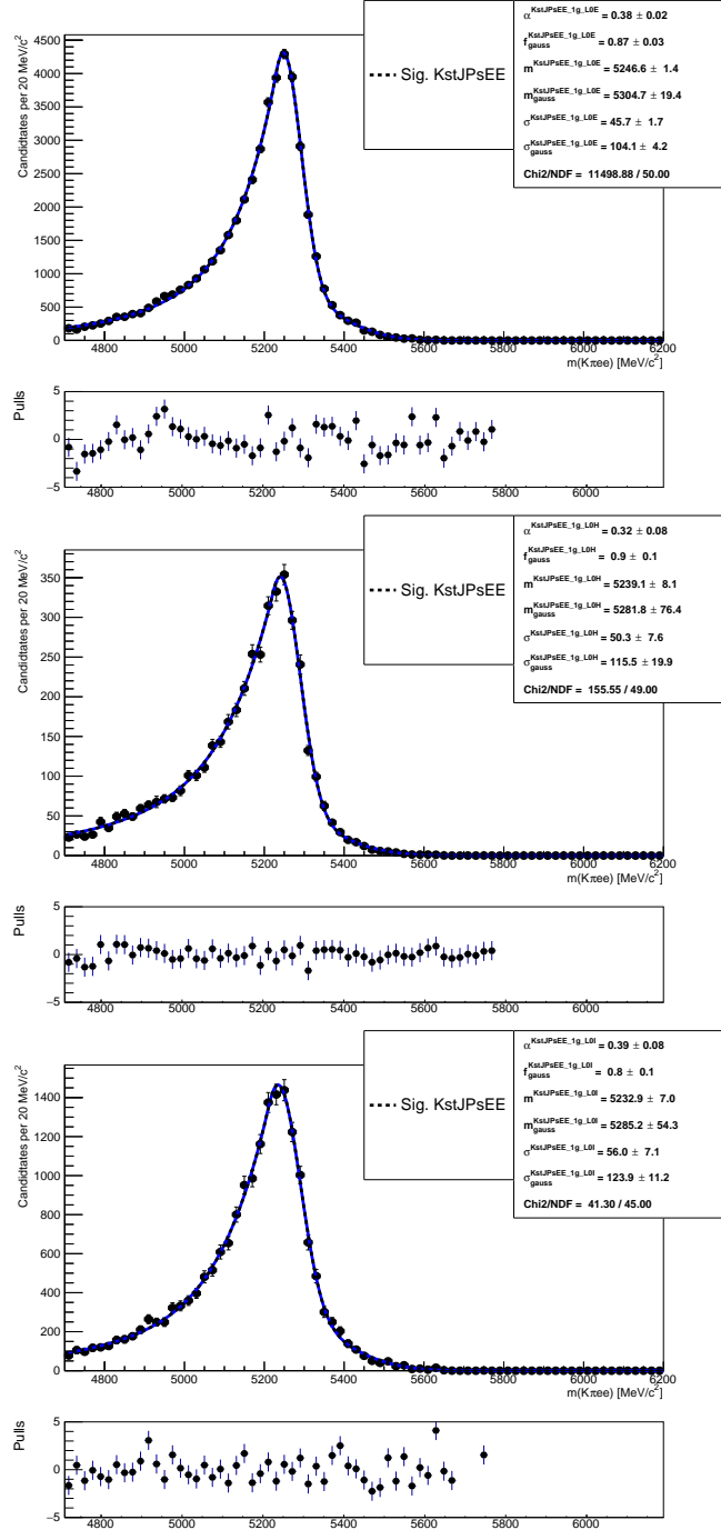
Figure G.3: Fitted m(K\pi\pi e) mass spectrum of B^0 \rightarrow K^{*0} J/\psi (J/\psi \rightarrow ee) simulated events in the three trigger categories and one photon emitted.
