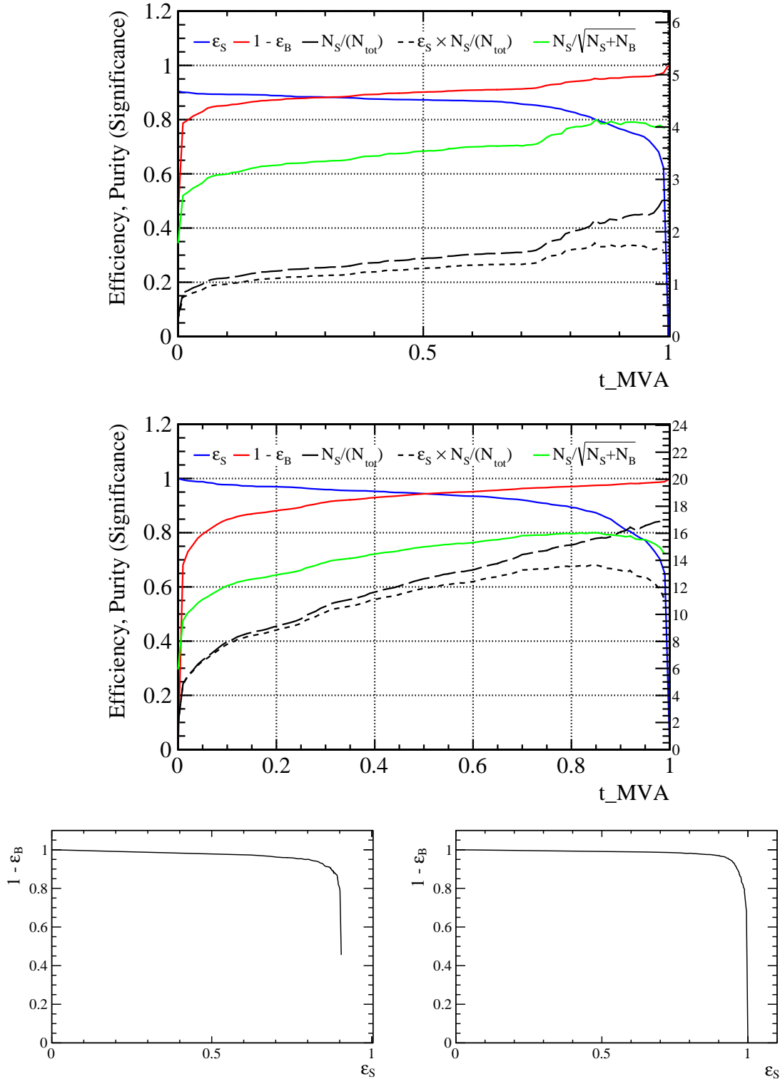
Figure 5.16: Dependence of figure-of-merit on the requirement on neural network output for electrons (top) and muons (middle). At the bottom, signal efficiency versus background rejection. Plots correspond to the electron (left) and muons (right) samples.
