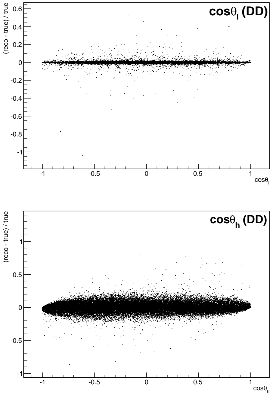
Figure 4.3: Difference between generated and reconstructed angular observables as a function of the observables themselves for downstream candidates: for \cos\theta_l (top) and \cos\theta_h (bottom). The spread of these distributions can be interpreted as the angular resolution.
