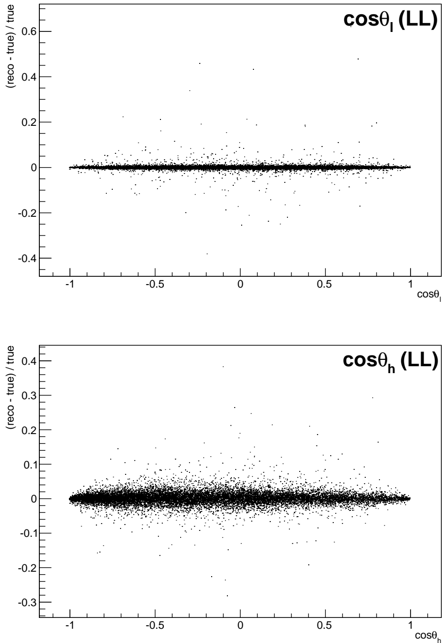
Figure 4.2: Difference between generated and reconstructed angular observables as a function of the observables themselves for long candidates: for \cos\theta_\ell (top) and \cos\theta_h (bottom). The spread of these distributions can be interpreted as the angular resolution.
