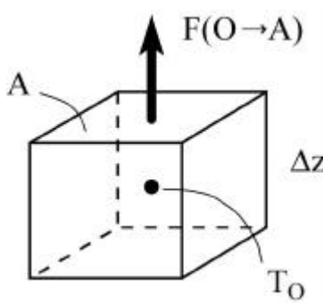
Figur 8.4: 1-Box Modell zur Illustration von restoring fluxes.
