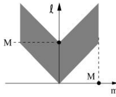
Figur 6.7b: Rhomboidal truncation
