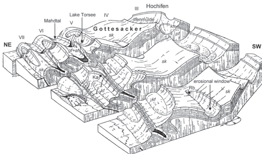
Fig. 4. Block diagram of the Hochifen-Gottesacker area, view from NW. Lithostratigraphy (formations): Palfris (pf), Kieselkalk (kf), Drusberg (df), Schratenkalk (sk), Garschella (gf), and Amden (af), Quaternary deposits (q). Geological structures: Anticlines in roman numerals. An important NE-trending left-lateral strike-slip fault cuts through anticlines V-VII. Hydrology: Lake Torsee, Kessleralp spring (Ka), Rubach (Rb) spring (Wagner 1950, supplemented).
