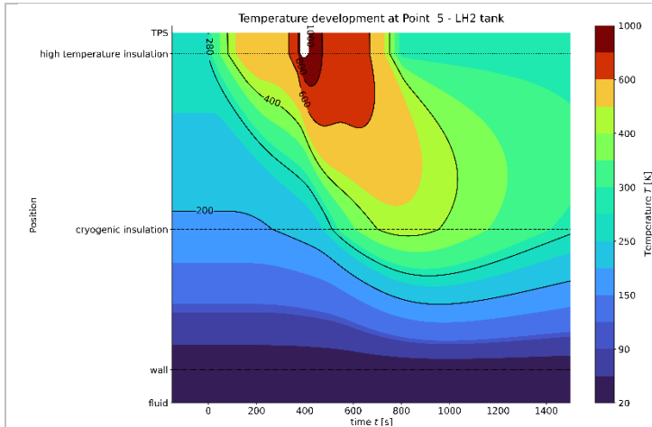
Figure 1: Exemplary evolution of temperature over time for an architecture without purge gap consisting of an external cryogenic insulation (PU-foam, 20mm) and a high temperature insulation (altramat, 25mm) and an external panel (CMC, 3mm)
