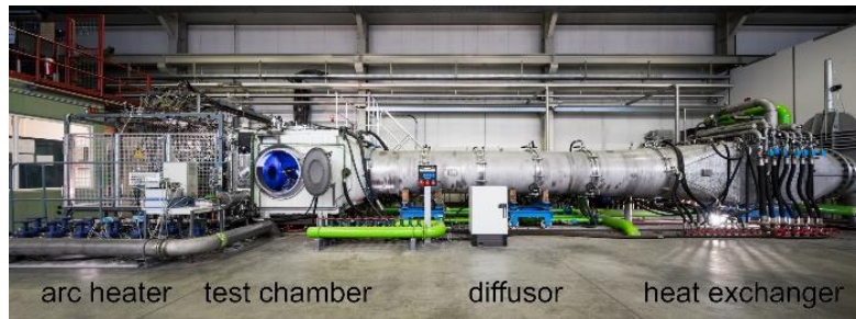
Figure 12: Arc-Heated Wind Tunnel L3K [13]
