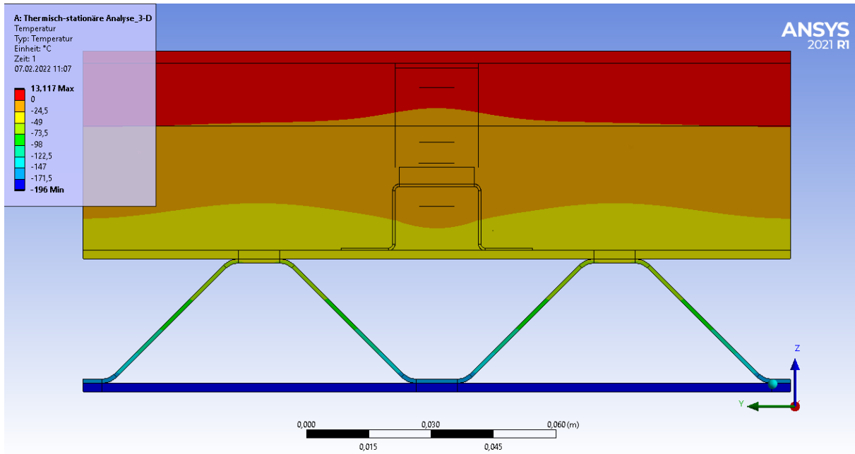
Figure 9: Temperature contours within the ITO under thermal steady-state conditions with liquid nitrogen as cryogenic propellant substitute.
