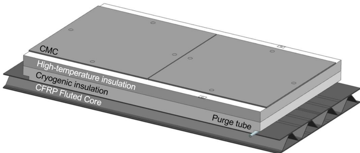
Figure 8: Concept of the ITO.
