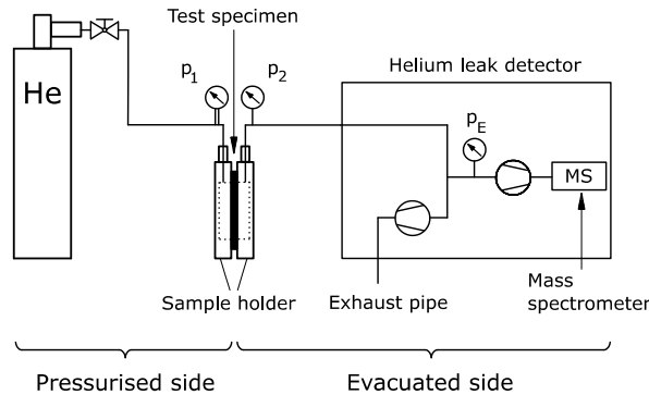
Figure 10: Scheme of the permeation test rig.
