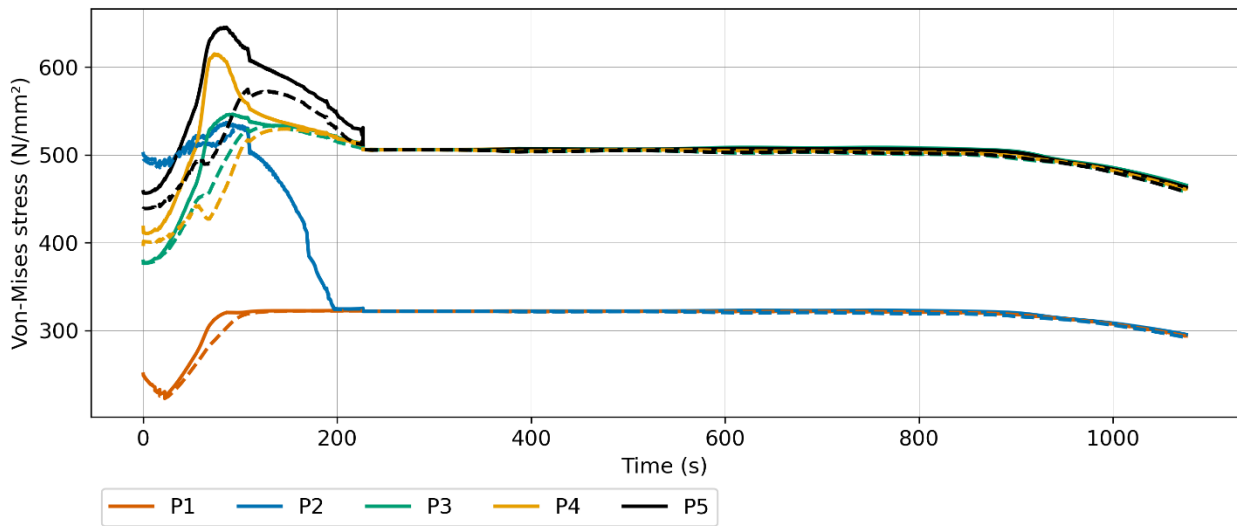
Figure 5: Von-Mises stress of the SpaceLiner booster on tension (dashed) and compression side (solid) at points P1 (front of oxygen tank) to P5 (back of hydrogen tank)
