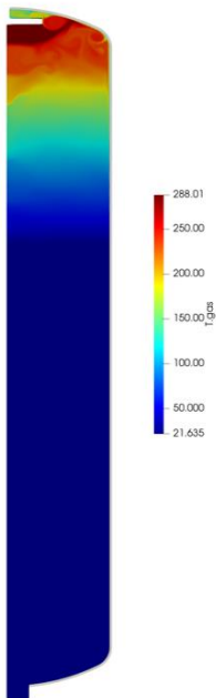
Figure 6: Thermal stratification during propellant pressurization
