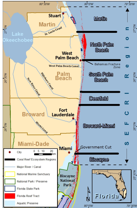
Figure 1. Study area included all hardbottom and reef habitats between the northern boundary of Martin County to Government Cut in Miami-Dade County.
