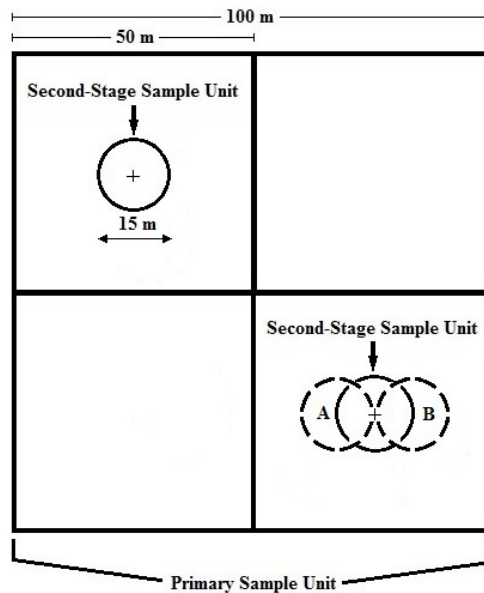
Figure 2. Illustration of Primary Sample Unit (PSU) and Second-Stage Sample Units (SSUs). Selection of 2 individual target SSUs was accomplished by a randomization of the 4 cells within the PSU. The dashed circles represent a buddy pair (A and B). [modified from Smith et al., 2011]
