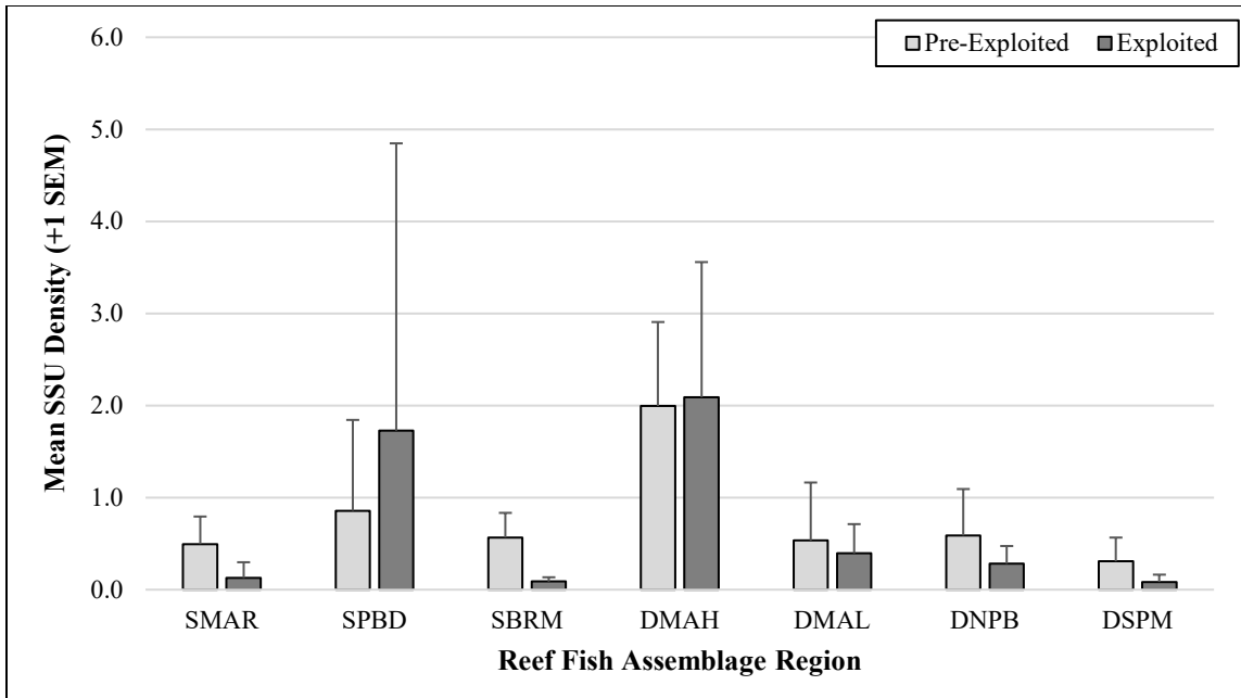
Figure 26. Mean SSU density of Gray Snapper by Reef Fish Assemblage Region; pre-exploited and exploited life-stage comparison with all years combined.
