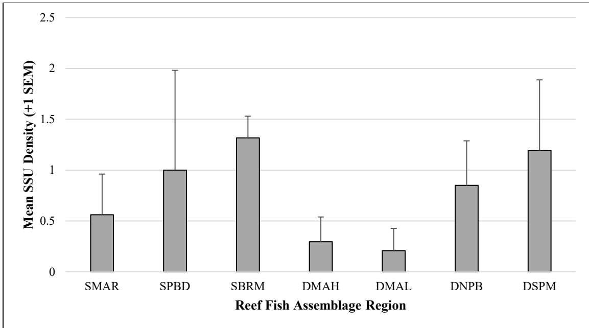
Figure 32. Yellowtail Snapper mean SSU density by Reef Fish Assemblage Region, with all years combined.
