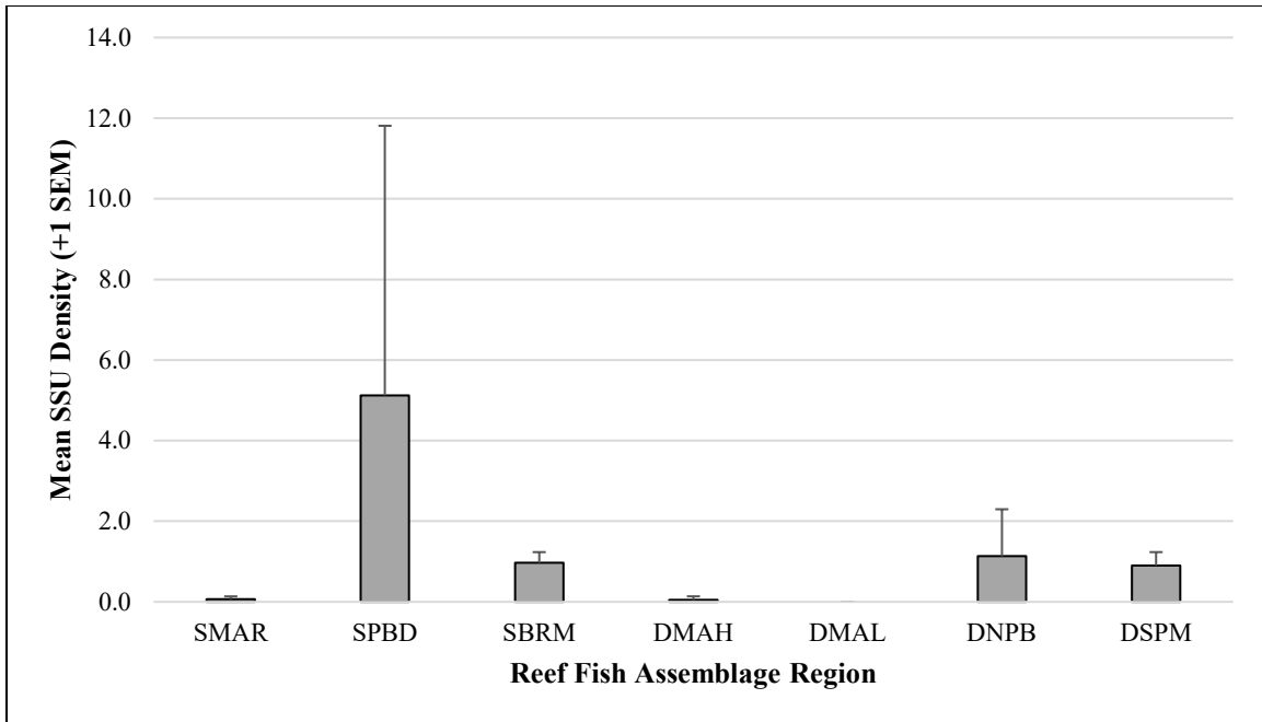
Figure 46. Bluestriped Grunt mean SSU density by Reef Fish Assemblage Region, with all years combined.
