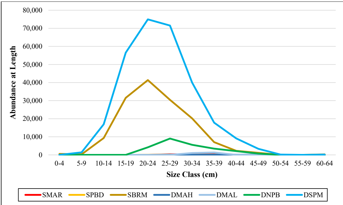
Figure 57. Length frequency comparison for Hogfish by total estimated assemblage region-wide population size (abundance at length) for southeast Florida, with all years combined.
