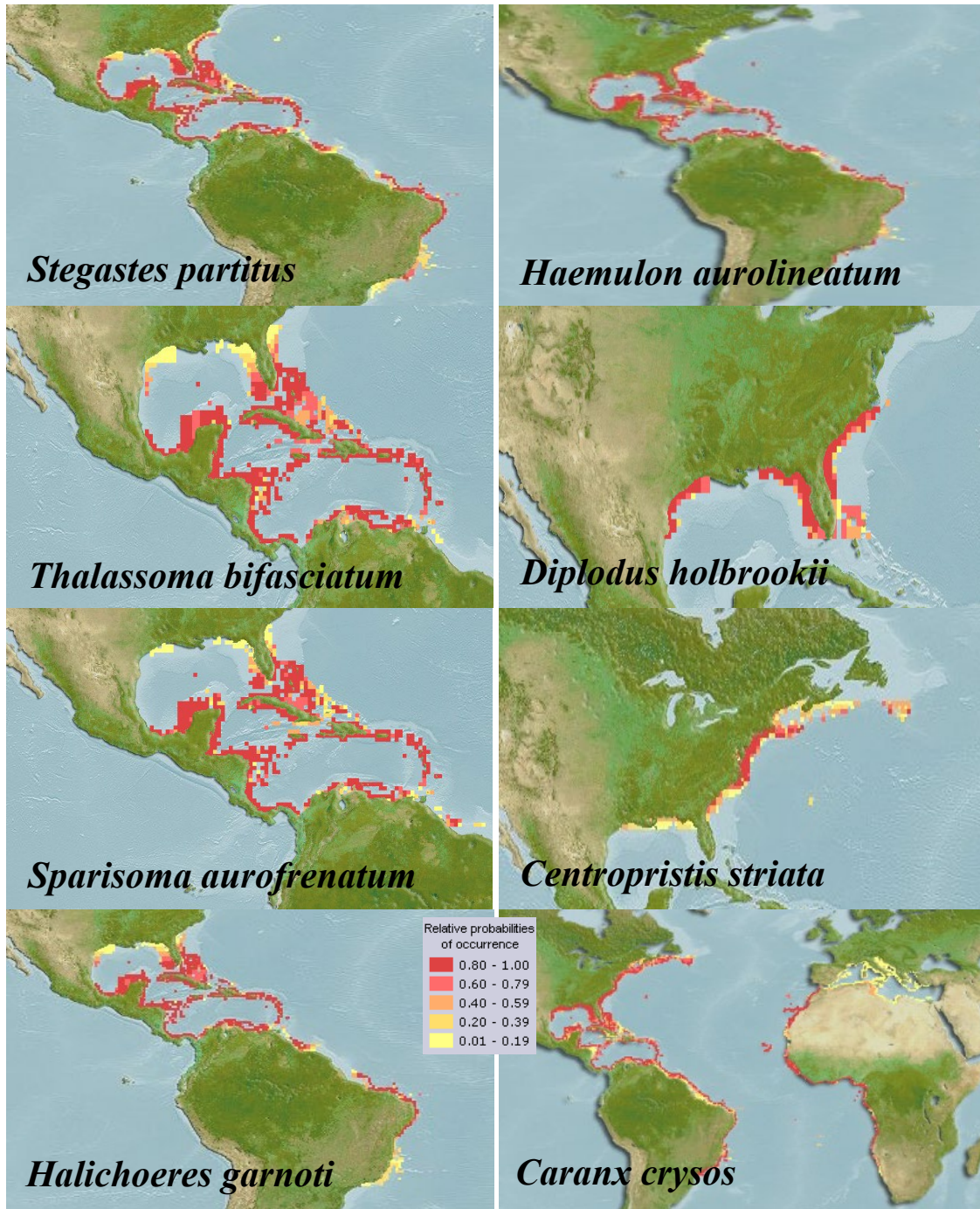
Figure 7. Examples of known ranges for some of the species driving the differences in assemblages between the southernmost Broward-Miami region and the northernmost Martin region (Kaschener et al., 2013).
