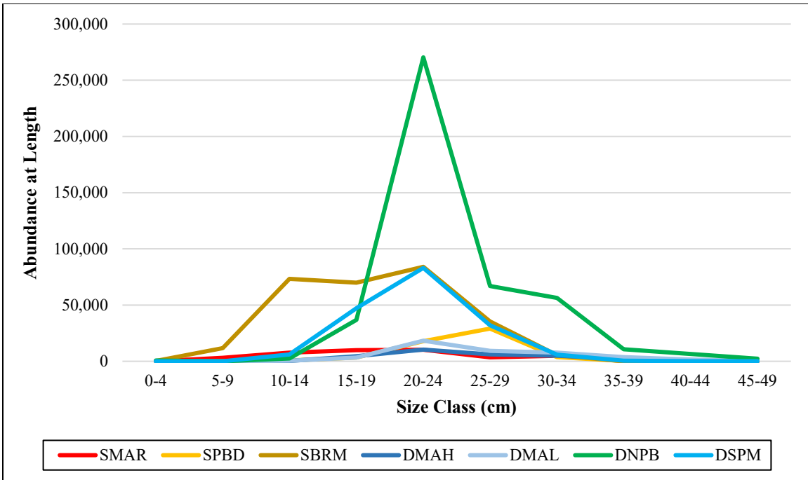
Figure 28. Length frequency comparison for Gray Snapper by total estimated assemblage region-wide population size (abundance at length) for southeast Florida, with all years combined.
