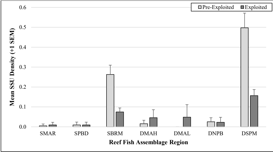
Figure 55. Mean SSU density of Hogfish by Reef Fish Assemblage Region; pre-exploited and exploited life-stage comparison with all years combined.
