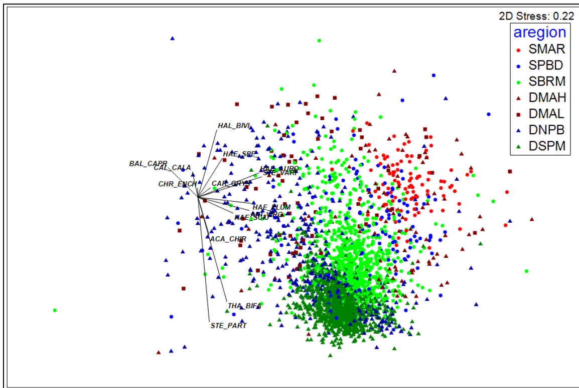
Figure 5. MDS plot of all sites (2012 – 2016) categorized by Reef Fish Assemblage Region. “S” indicates Shallow ( \leq 10 m) and “D” indicates Deep ( > 10 m) assemblage regions. Shallow sites are denoted by solid circles and the Deep sites are solid triangles. Solid squares are Deep Low Relief. Lines indicate Pearson correlations of select species (chosen from SIMPER analyses) showing their influence on site similarities in the plot.
