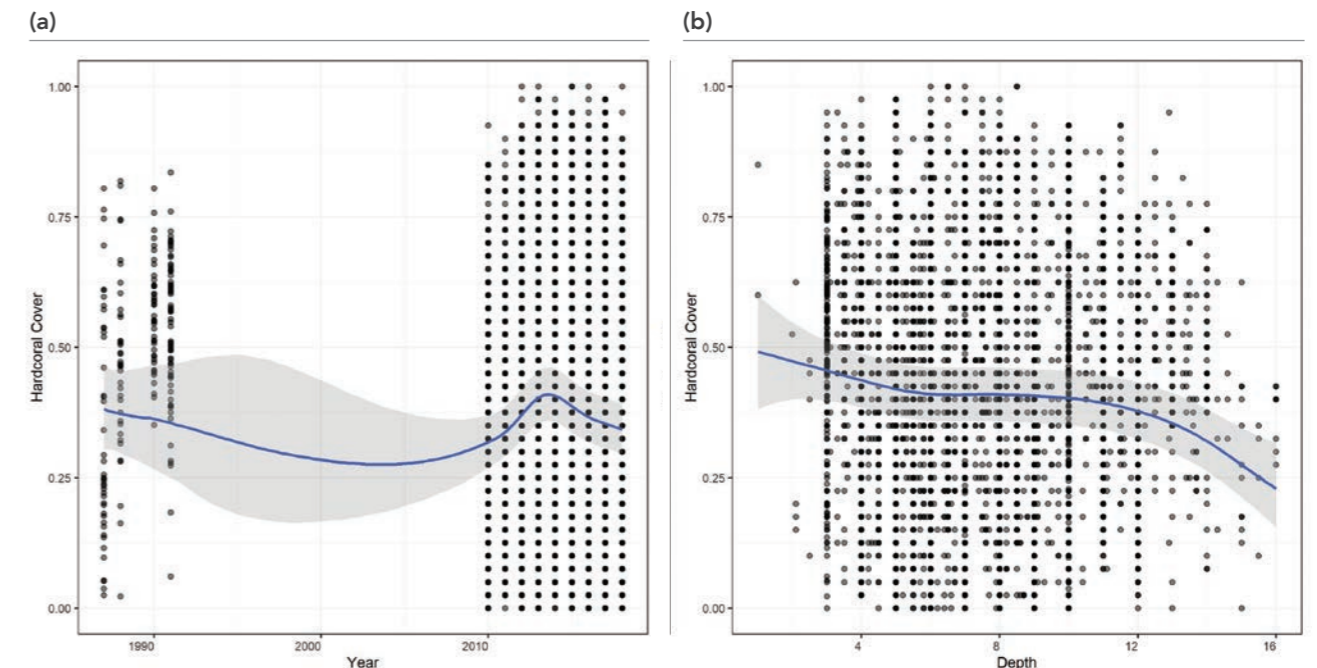
FIGURE 2: Malaysia coral cover across (a) years and (b) depths.
