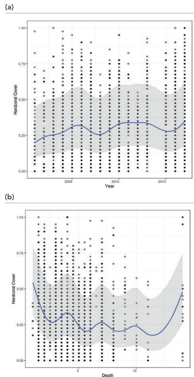
FIGURE 2: Vietnam coral cover across (a) years and (b) depths.
