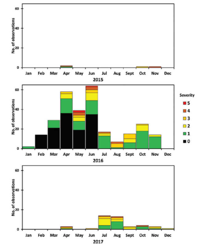
FIGURE 4: (A) Extent and severity of coral bleaching incidence (or the absence of) from 2015 to 2017 in the Philippines; (B) Summary of coral bleaching and no bleaching reports submitted to PCBW from 2015 to 2017.
