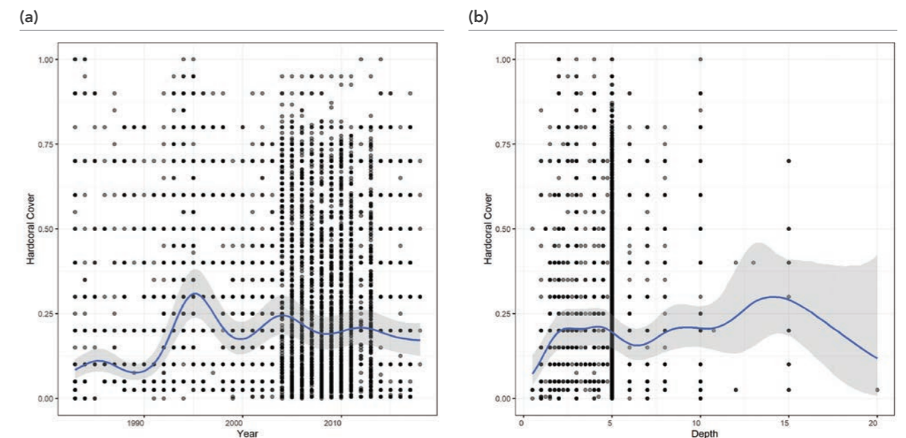
FIGURE 2: Trends in coral cover in Japan across (a) years and (b) depths.
