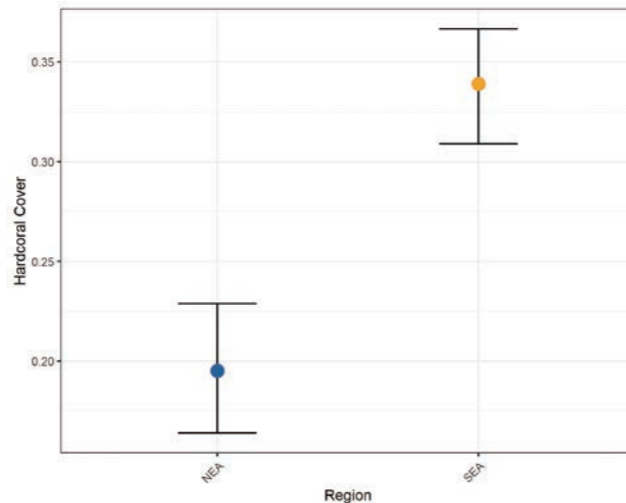
FIGURE 10: Regional level variation in coral cover based on the Bayesian HGAMs, showing much lower mean coral cover in Northeast Asia (NEA) compared to Southeast Asia (SEA) though with similar levels of variation.
