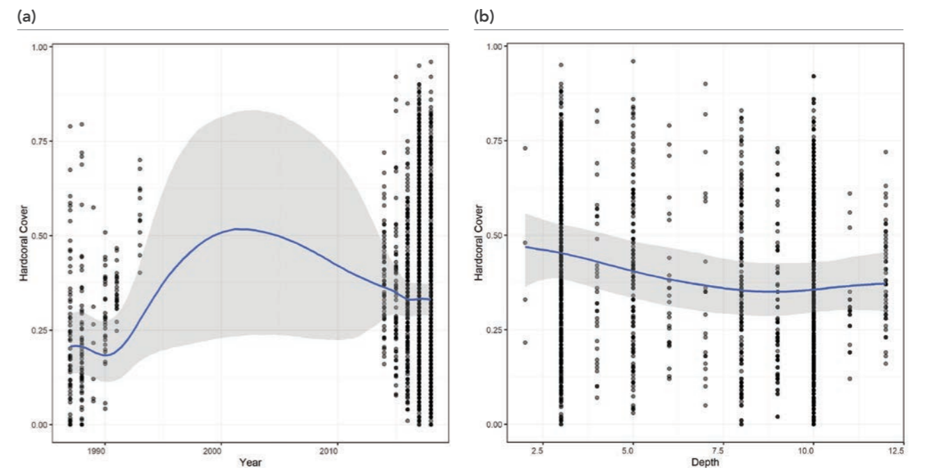
FIGURE 2: Indonesia coral cover across (a) years and (b) depths.
