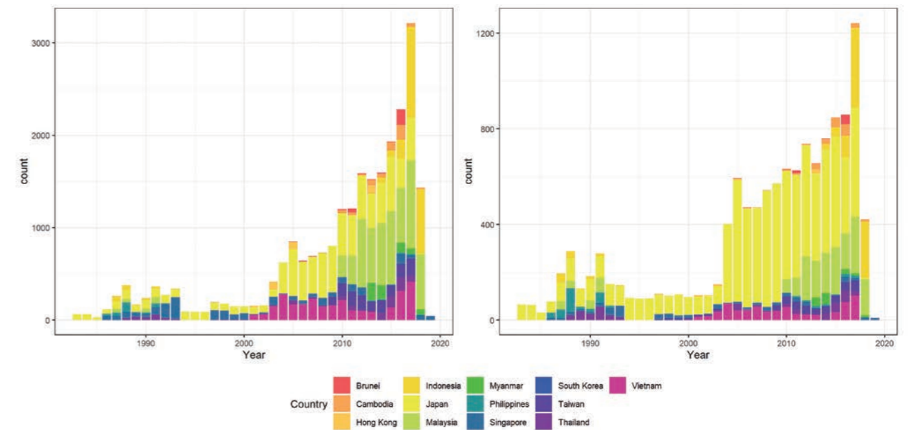
FIGURE 4: Stacked bar plots of unique surveys (left) and transects (right) by year and colored by countries, showing large increases of both surveys and transects after the year 2000 across the different countries and regions.
