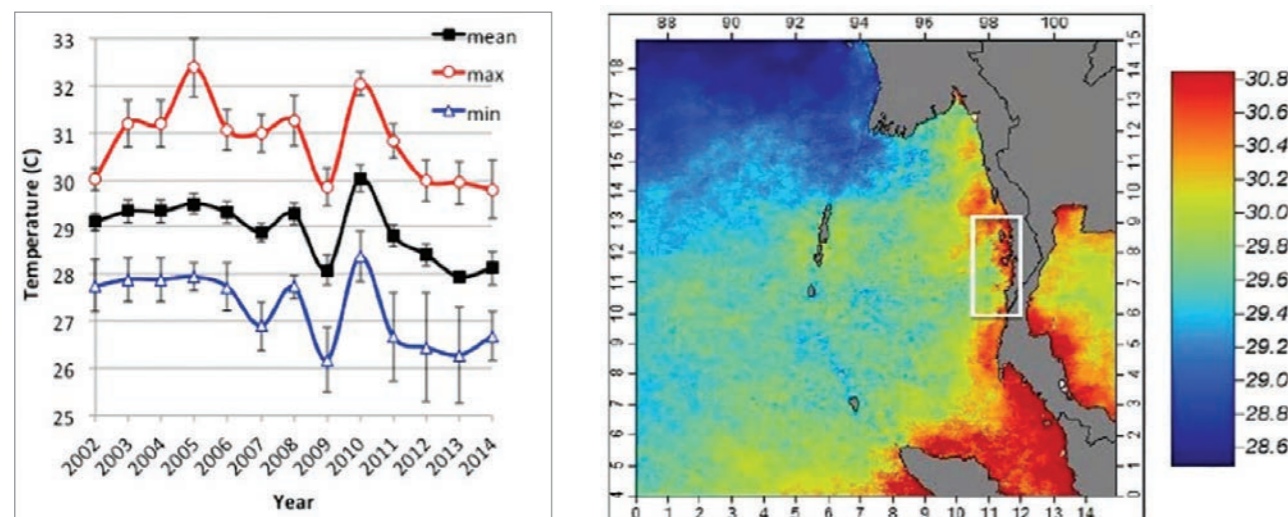
FIGURE 8: (Left) Sea surface temperature in the Myeik Archipelago, from 2002 to 2014, using MODIS 4 km resolution data, showing monthly mean, maxima and minima across 24 sampled points. (Right) Mean monthly temperature for 2010. The approximate location of the archipelago and survey locations is shown by the white rectangle.
