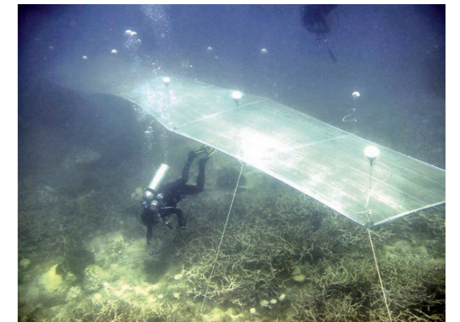
FIGURE 4: A field shading experiment at Mu Ko Chumphon National Park, the Western Gulf of Thailand.
