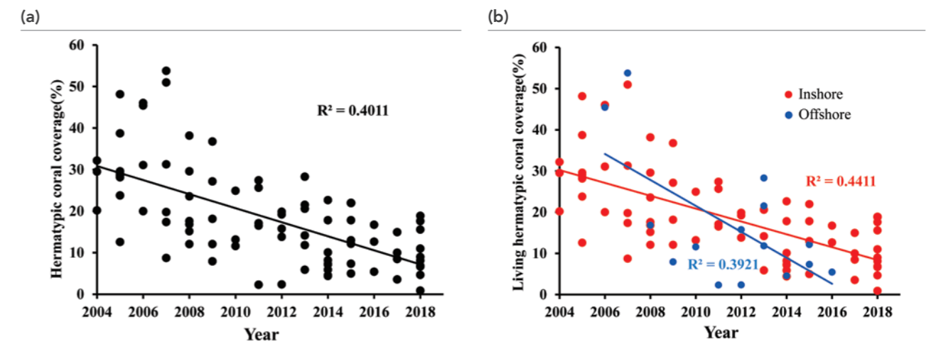
FIGURE 3: (a) Changes in coverage of live hermatypic corals in China; (b) Changes in coverage of live hermatypic corals between inshore and offshore locations in China.
