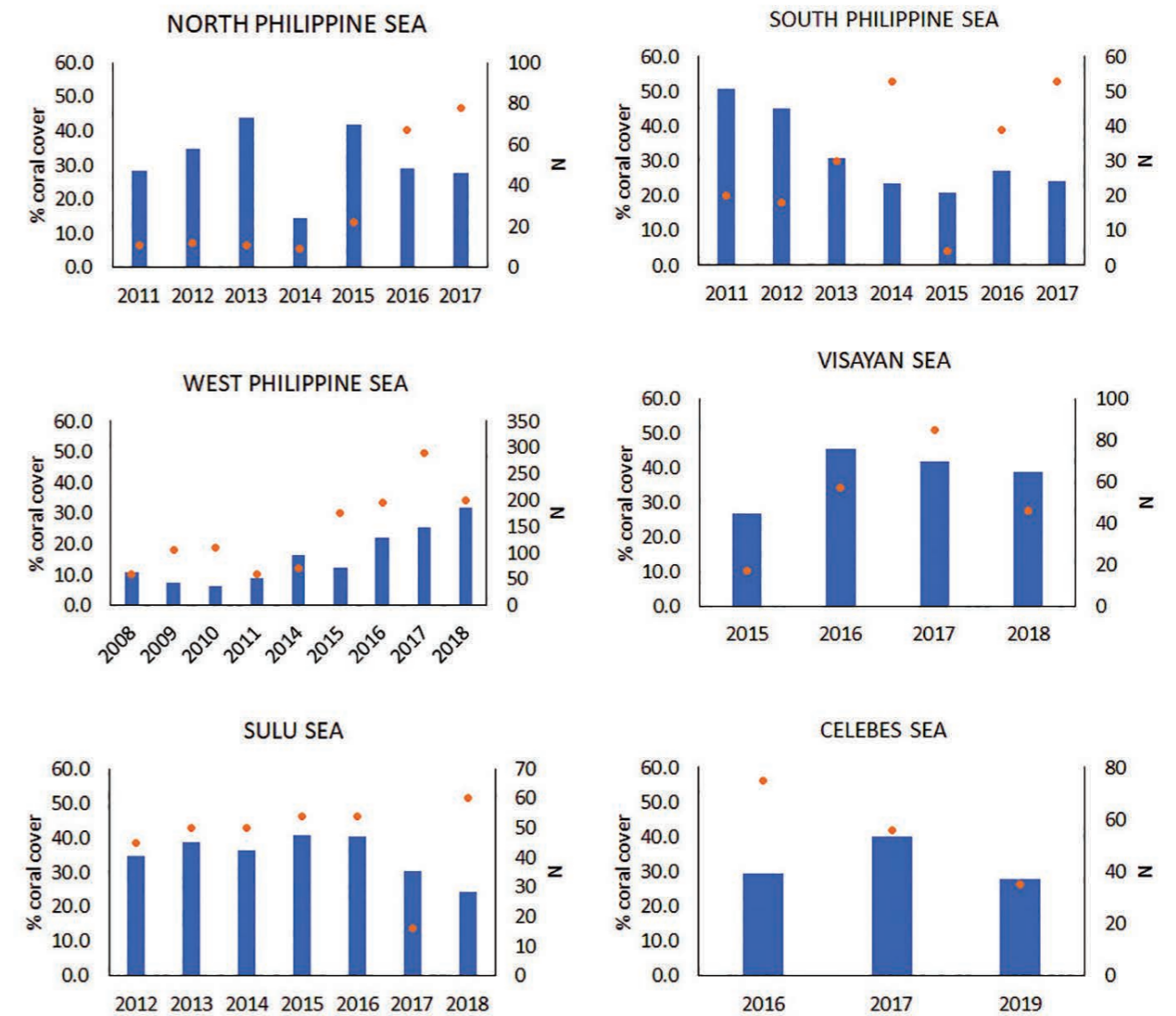
FIGURE 2: Percent coral cover (hard and soft corals) of Philippine reefs across biogeographic regions through time. N represents the total number of transects used in LIT and photo quadrats inside and outside the Marine Protected Areas (MPAs).
