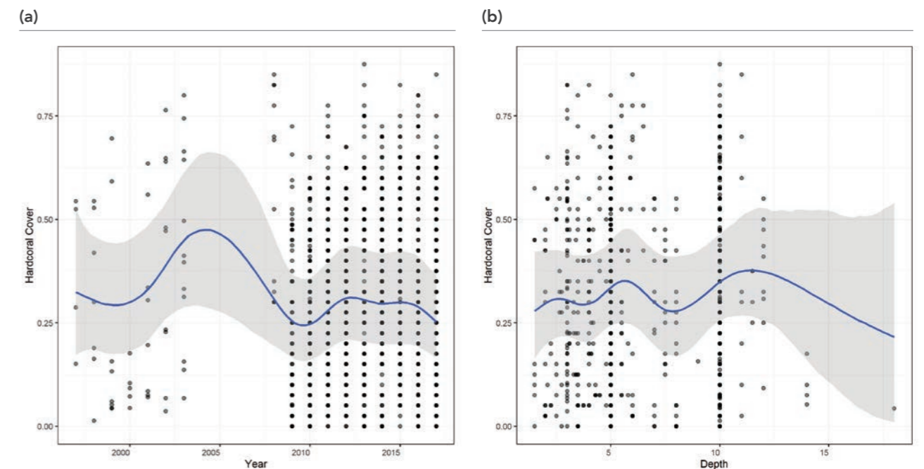
FIGURE 3: Taiwan coral cover across (a) years and (b) depths.
