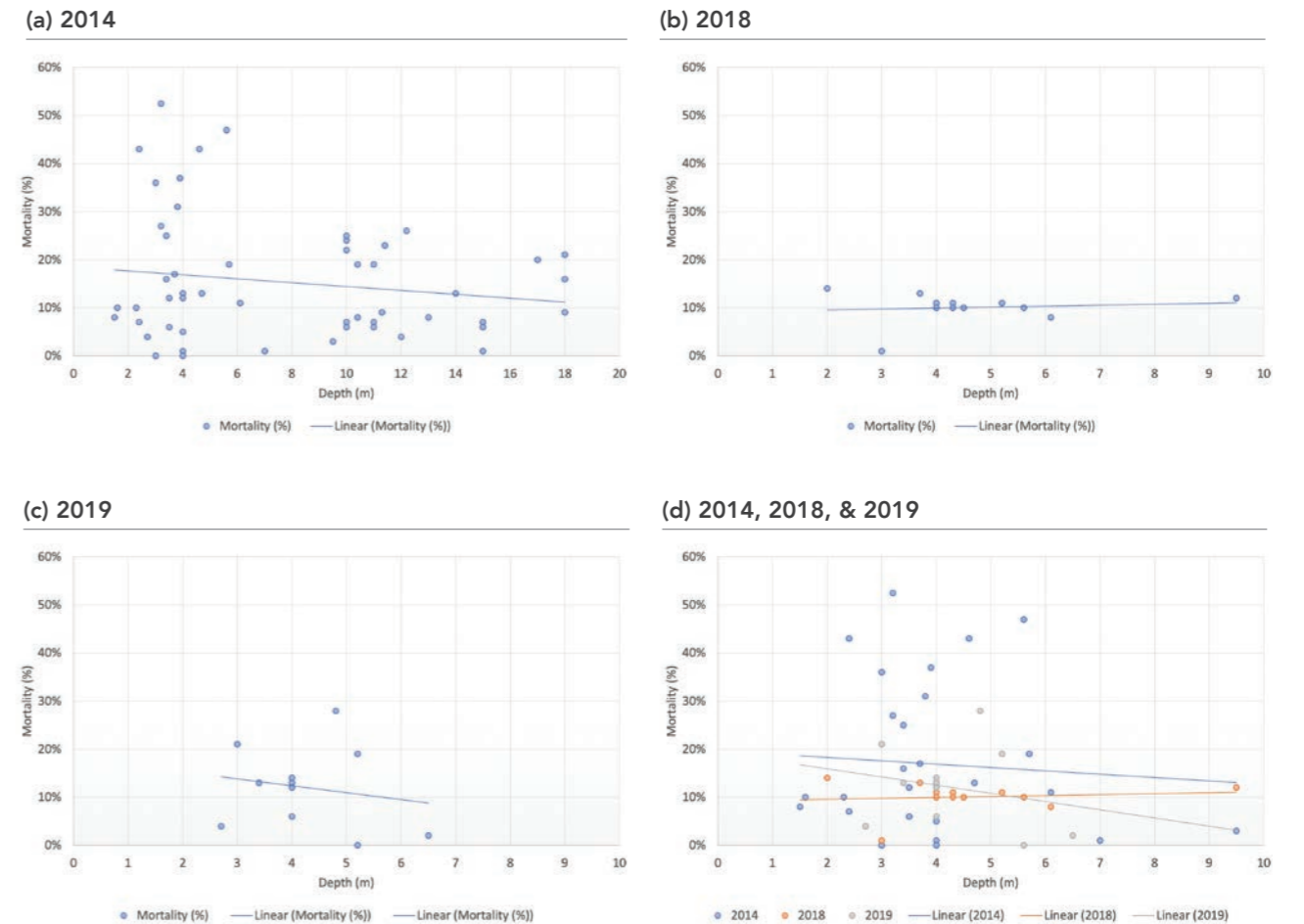
FIGURE 6: Coral mortality percentage; (a), (b) and (c) for yearly mortality in percentage; (d) for coral mortality percentage comparison between years.
