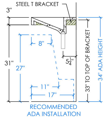
RIGHT SECTION
