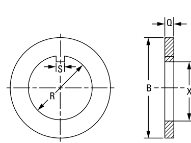
Fig. 54. Tongued washers.
