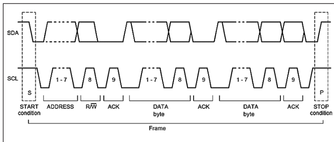
Abb. 12.4: I 2 C 7-Bit-Adresse
