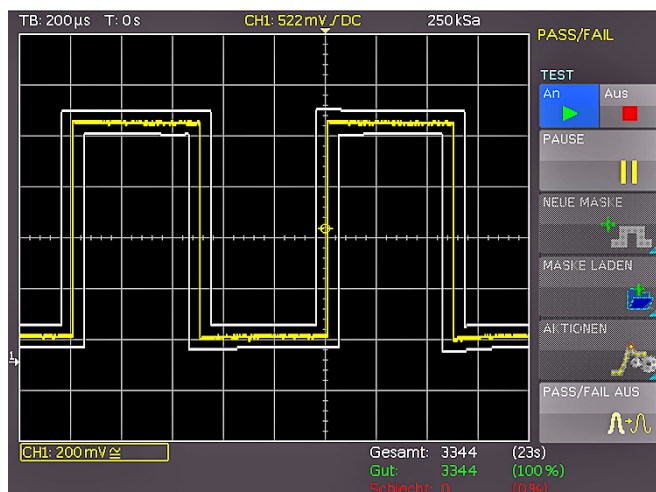
Abb. 9.9: PASS/FAIL Maskentest
