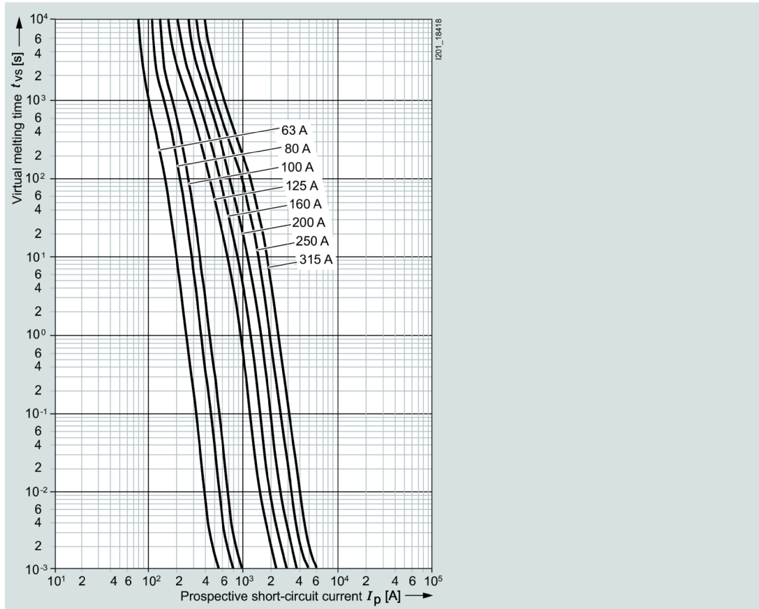
Time/current characteristic curves diagram 1500 V
