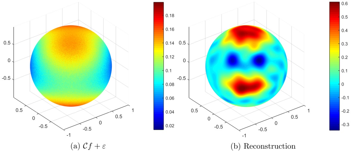
Figure 6: Cosine transform of the function from Figure 2a and its reconstruction. The left image shows the cosine transform with added random noise \varepsilon that has a variance of \sigma = 0.01 and the right image the reconstruction given from M = 520\,000 data points.
