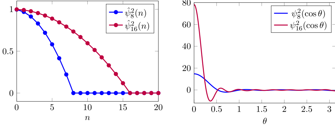
Figure 1: The mollifiers \psi_{\tilde{N}}^s from Definition 3.3 are illustrated for s = 2 and \tilde{N} \in \{8, 16\} . The left image shows their Fourier coefficients, and the right one shows their function values depending on the polar angle \theta .
