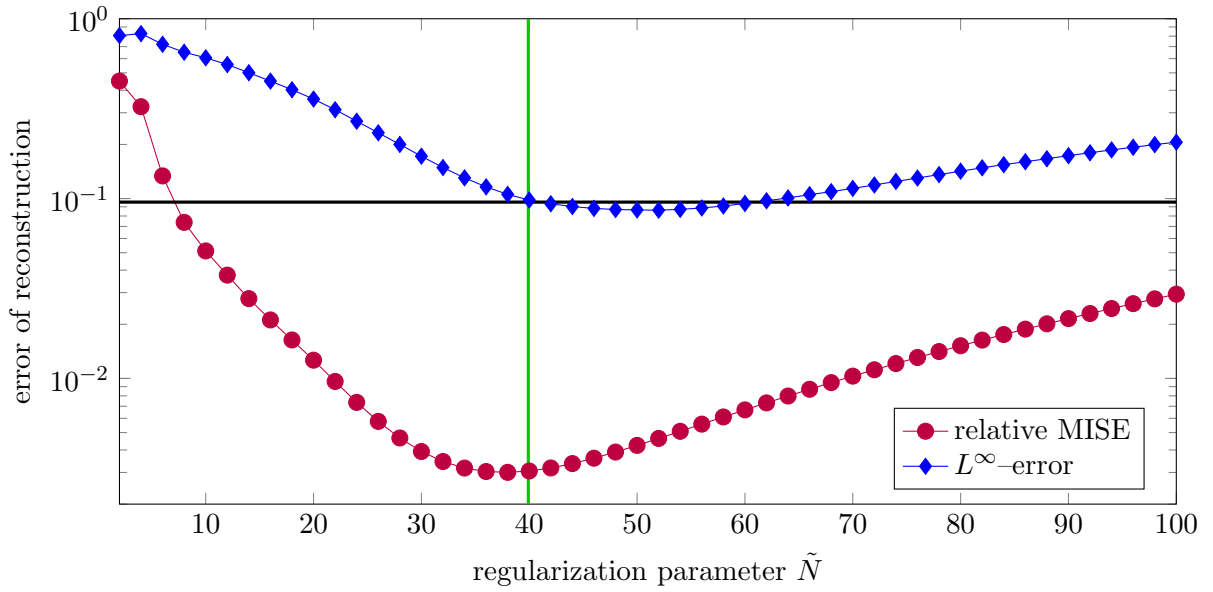
Figure 5: Error of the reconstruction from M = 520\,000 data points ( N = 500 ) with respect to the regularization parameter \tilde{N} . The green line indicates the computed value \tilde{N}^* from (3.17). The black line indicates the minimax (3.18) of the relative MISE for \tilde{N} = \tilde{N}^* .
