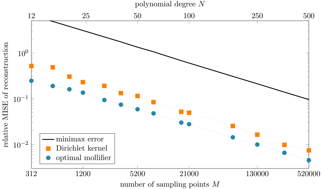
Figure 4: Log–log plot of the relative MISE \|f - \mathcal{E}(\mathcal{F}f + \varepsilon)\|_{L^2} / \|f\|_{L^2} for the reconstruction of the test function f depicted in Figure 2a from its Funk–Radon transform perturbed by white noise \varepsilon , signal-to-noise ratio 2.6dB, with respect to the number M of sampling points. The blue circles represent the results using the optimal mollifier \psi_N^s and the orange squares represent the results using the Dirichlet kernel \psi_N^{\text{Dir}} . The black line shows the theoretic minimax rate (3.18) for functions within the same Sobolev ball as the test function f .
