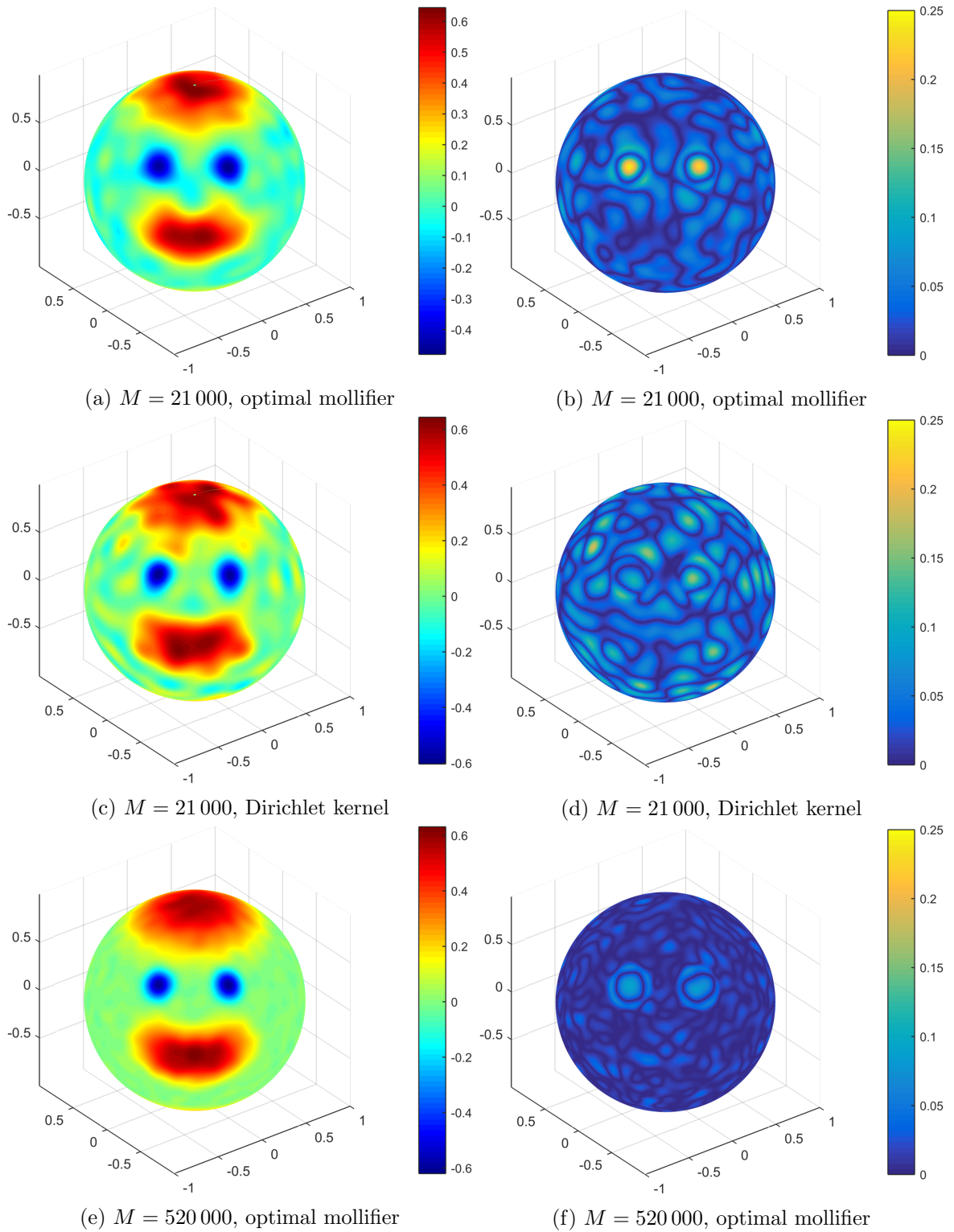
Figure 3: Reconstruction results \mathcal{E}_{N,\psi_N^2}(\mathcal{F}f + \varepsilon) (left) and the respective errors |f - \mathcal{E}_{N,\psi_N^2}(\mathcal{F}f + \varepsilon)| (right) for different amounts M of sampling points and different mollifiers.
