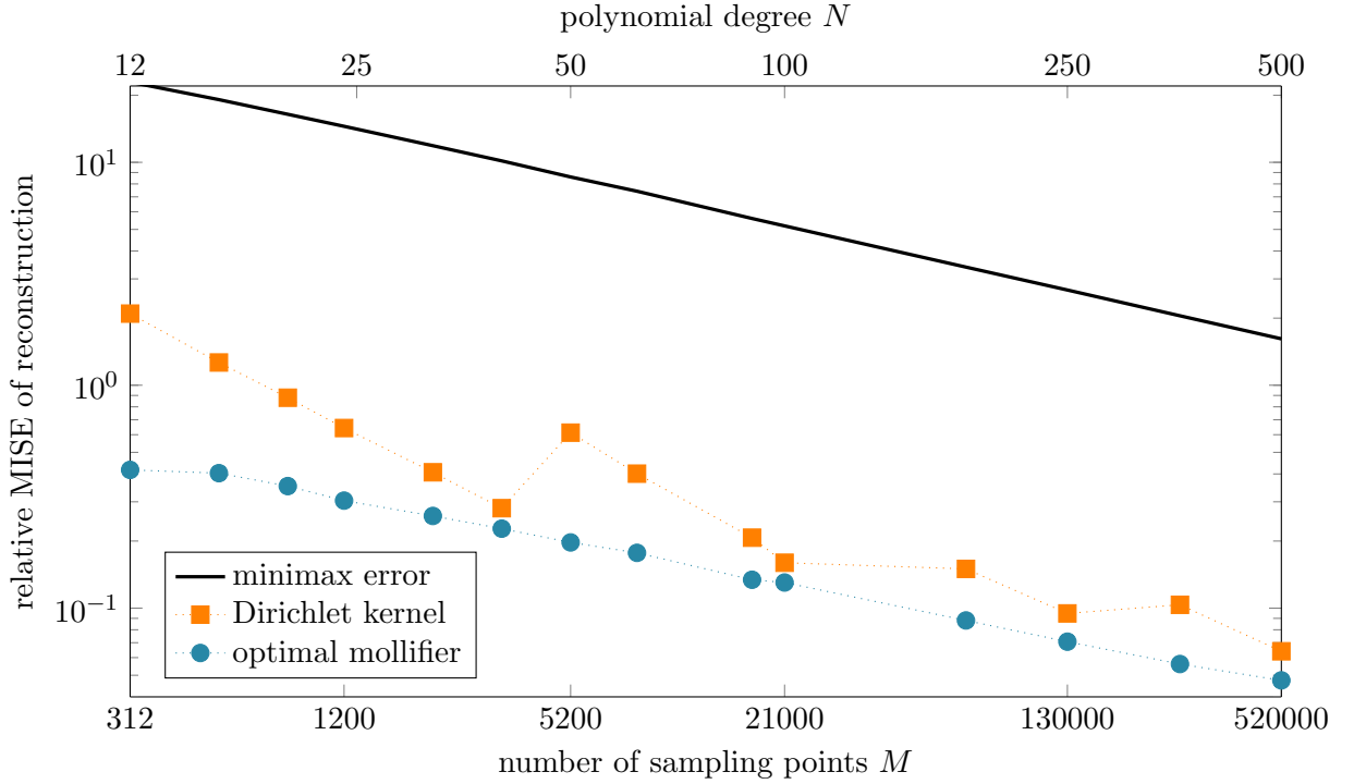
Figure 7: Log–log plot of the relative MISE \|f - \mathcal{E}(\mathcal{C}f + \varepsilon)\|_{L^2}/\|f\|_{L^2} for the reconstruction of the test function f depicted in Figure 2a from its cosine transform perturbed by white noise \varepsilon , signal-to-noise ratio 21dB, with respect to the number M of sampling points. The blue circles represent the results using the optimal mollifier \psi_{\tilde{N}}^s and the orange squares represent the results using the Dirichlet kernel \psi_{\tilde{N}}^{\text{Dir}} . The black line shows the theoretic minimax rate (3.19) for functions within the same Sobolev ball as the test function f .
