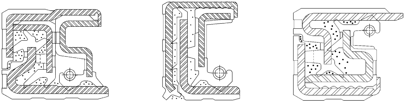
Figure 31: AP Style Seals
