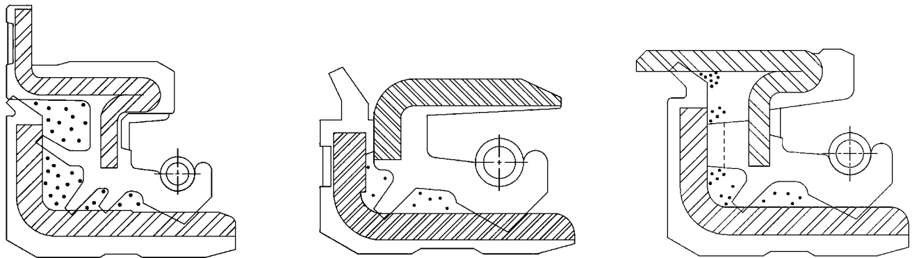
Figure 30: AO Style Seals
