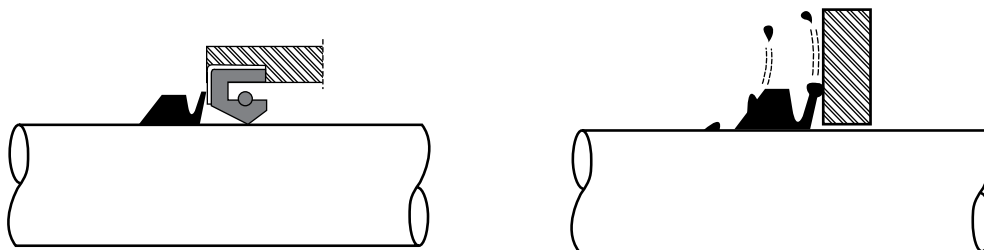
Figure 22: V-Ring Functions
