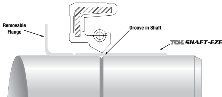
Figure 34: Shaft-Eze Function
