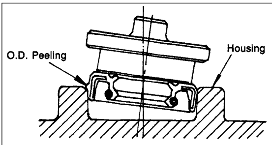
Figure 13: Misalignment Error
