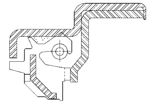
Figure 27: ST Style Oil Bath Seal
