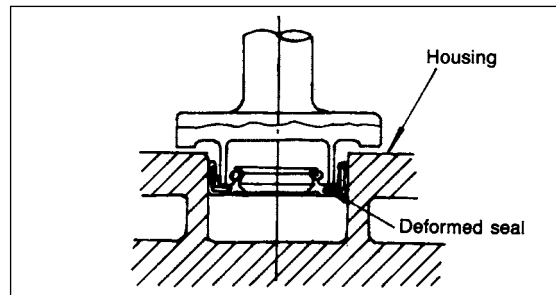
Figure 14: Deformed Seal
