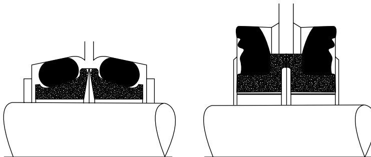
Figure 32: Track Roller Seals
