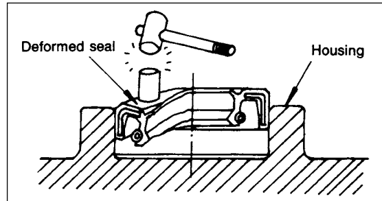
Figure 12: Deformed Seal
