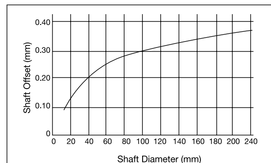
Figure 2: Shaft-To-Bore-Misalignment
