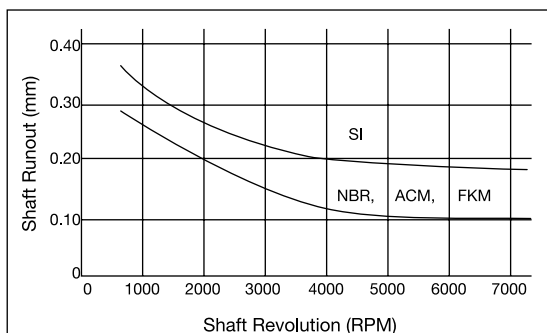
Figure 1: Dynamic Runout
