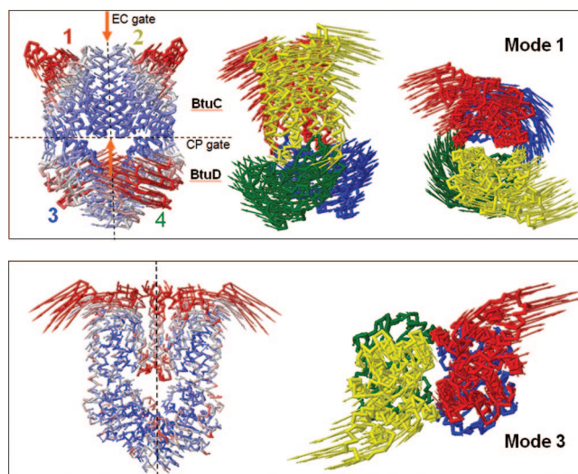
Figure 20. Global dynamics of the ABC transporter BtuCD. Top and bottom panels display the collective motions of the tetramer in the ANM modes 1 and 3, respectively, recently examined by Weng et al. (2008). The color-coded diagrams on the left in both panels display the size of motions (red, most mobile; blue, almost rigid) induced in these modes. The other diagrams display the relative motions of the two TM domains (1, red; 2, yellow) of the BtuC dimer, and the two NBDs (3, blue; 4, green) of the BtuD dimer, that compose the BtuCD tetramer, viewed from the side ( middle diagram in top panel) or from the EC region ( right diagrams in both panel). The two gates (EC and CP gates) of the substrate (vitamin B 12 ) translocation pore are indicated by the orange arrows in the left diagram of the top panel.
