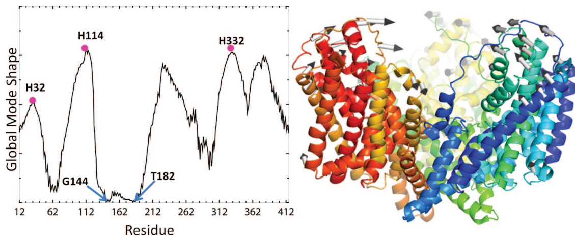
Figure 19. Global dynamics of the aspartate transporter Glt ph predicted by the ANM. (A) Distribution of square displacements of residues, (\Delta R_i)^2|_1 + (\Delta R_i)^2|_2 (see eq 26), induced in the asymmetric stretching–contraction mode (a 2-fold degenerate mode). The same profile is induced in all three subunits upon superposition of these two lowest frequency modes, leading to a cylindrically symmetric reconfiguration. Peaks refer to the most mobile residues, and minima to the hinge centers (e.g., Gly144 and T182) controlling the concerted movements of the subunits. The large amplitude swinging movements of the extracellular histidines suggest a possible role in facilitating the attraction of the anions or engulfing them into the central basin. (B) Mechanism of motion in the first nondegenerate ANM mode (see also panel C in Figure 18). The arrows indicate the direction of the concerted movements of the three subunits (note that the third subunit in the back is lightly visible).
