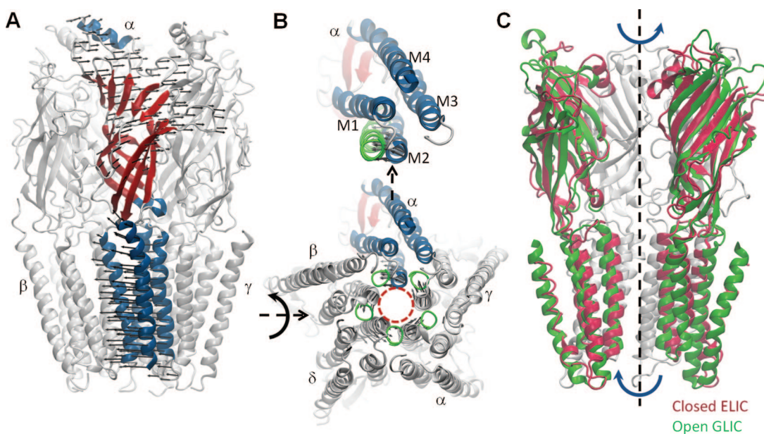
Figure 14. Ligand-gated ion channel nAChR structure and dynamics. (A) Structure of the EC and TM domains of nAChR 265 (PDB ID: 2BG9). The secondary structure of one of the monomers ( \alpha ) is colored to display the \beta -sandwich fold (red) of the EC domain and the four TM helices (M1–M4; blue) of the TM domain; and the remaining four monomers are shown in gray. The lowest frequency ANM mode induces a quaternary symmetric twist, as indicated by the arrows shown for monomer \alpha . (B) CP end of TM domain (bottom) and close up view of one of the monomers (monomer \alpha , colored) (top). Red dashed circle indicates the channel pore. Arrows indicate the collective movements of M2 helices along ANM mode 1. Green circles represent the CP end of the M2 helices after deformation along ANM mode 1. (C) Comparison of bacterial homopentameric LGICs ELIC (2VL0) and GLIC (3EAM) shows the contribution of this quaternary twist mode to the conformational changes involved in activation. One subunit (closest to the viewer) is omitted to display the channel pore.
