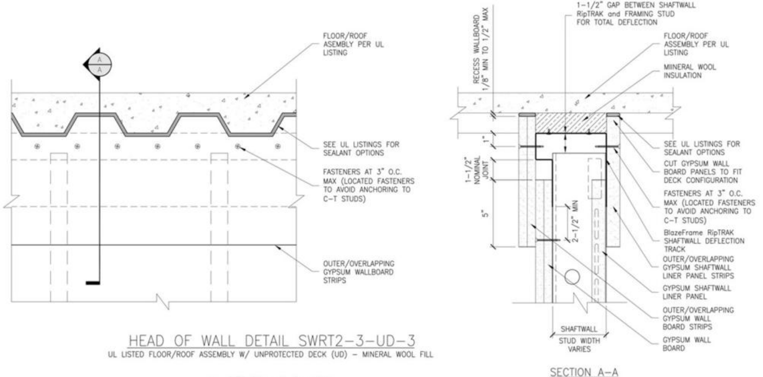
UL DESIGN HW-D-1141 (2 HR WITH 1-1/2" NOMINAL JOINT)
