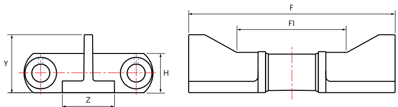
A Style Sharp Top Cradle Attachment
