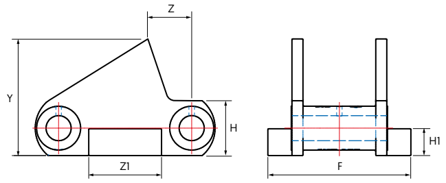
Integral S Pusher (integral guide blocks)
