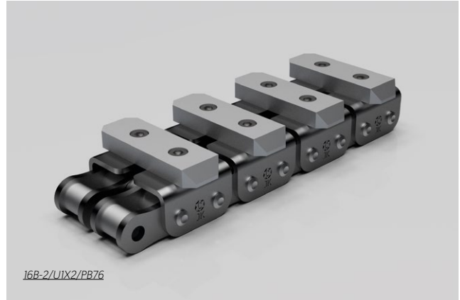
Aluminium Pad
