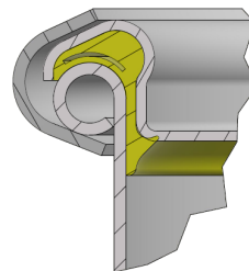
solution: MRC drum seal cavity filled design, dimensionally stable
