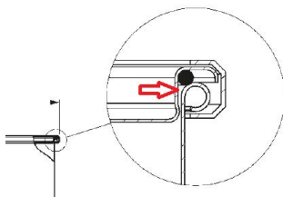
problem of standard drum lids: O-Ring seal with dead zones
