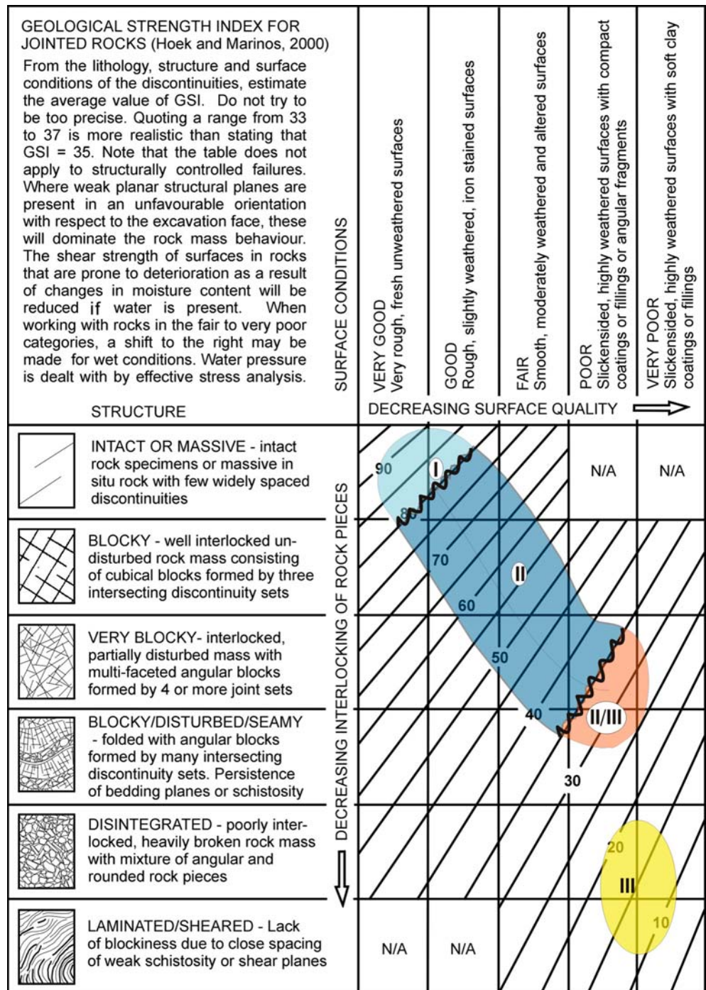
Fig. 17 Classification of the behaviour in tunnelling for peridotite–serpentinite rock masses in ophiolitic complexes (to be read in conjunction with Fig. 7)
