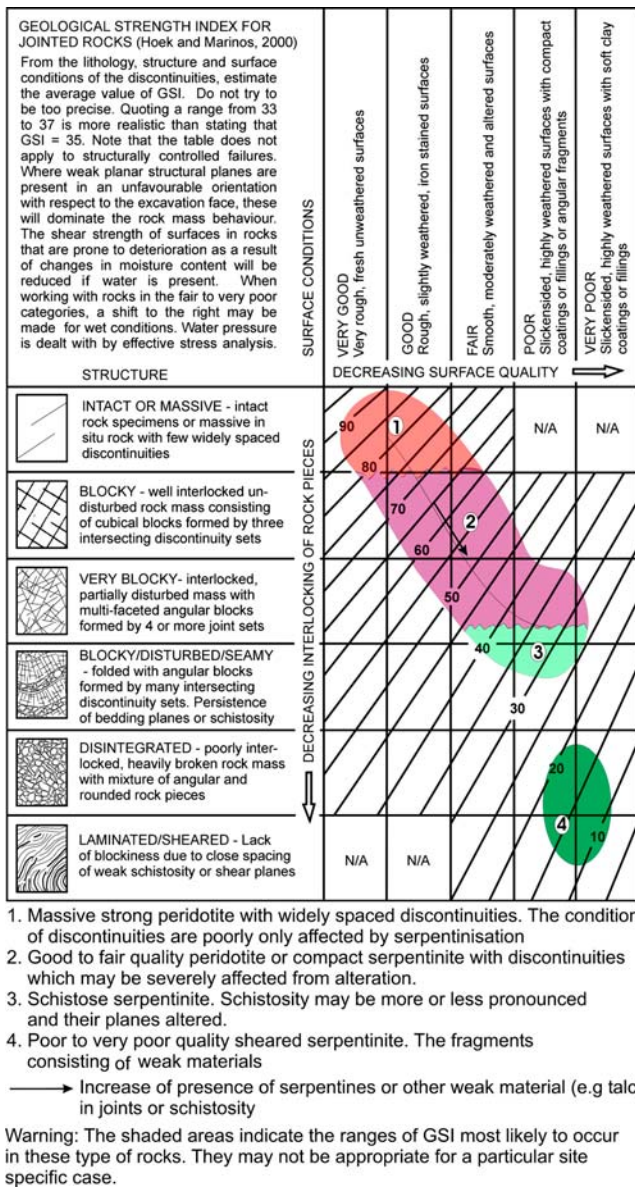
Fig. 7 Ranges of GSI for various qualities of peridotite–serpentinite rock masses in ophiolitic complexes
