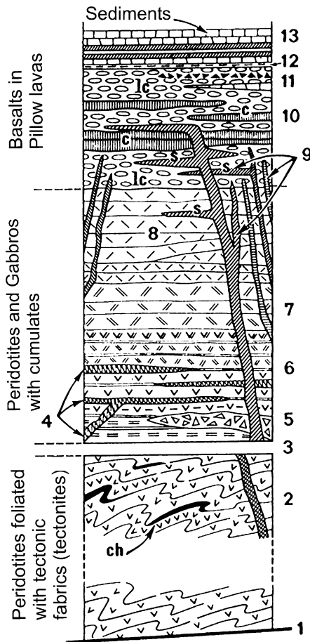
Fig. 2 Ophiolites: synthetic and theoretical column (from Foucault and Raoult 1995 with simplified descriptions). 1 basal contact, overthrust; 2 basal body of peridotites with foliation (tectonites), generally harzburgites with chromites ( ch ) layered with dunites; 3 tectonic cut or confused zone, 4 dykes, sills and layers of basic and ultrabasic rocks; 5 layered peridotites (cumulates of dunites, lherzolites) and magmatic breccia; 6 alternations of peridotites with gabbros, 7 non layered gabbros over layered gabbros, 8 variety of basic rocks, dolerites, diorites and granophyres (increase of \text{SiO}_2 ); 9 dykes, veins, sills ( s ) of basic rocks; 10 and 11 basalts (spilites) with compact flows ( c ) or pillow-lavas ( lc ), a tectonic contact is often present at the base of 10, 12 Argillites rich in Fe and Mn, 13 sedimentary rocks with siliceous beds (radiolarites) over or interlayered with the lavas (volcano-sedimentary complex). Total thickness: usually 4–5 km, can achieve 10–15 km (as an example: 11 and 10=0, 5–1 km, 8=0, 5 km, 7 and 6=0, 5 km, 5=0, 2 km, 2=2–3 km). These numbers can change dramatically due to overthrusts
