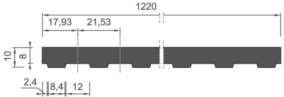
Profil EQUITONE [linea] Toleranz \pm 3 mm
