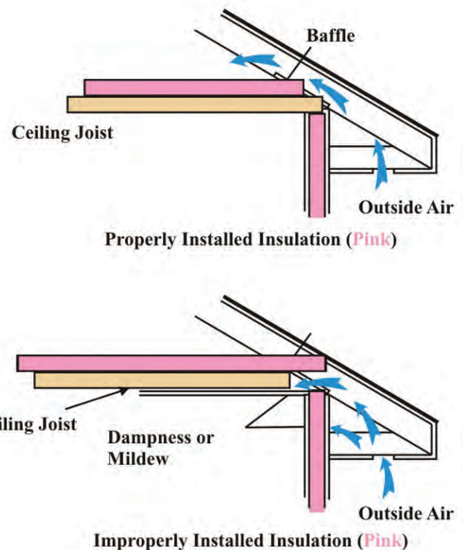
Figure 7.4. Attic ventilation
