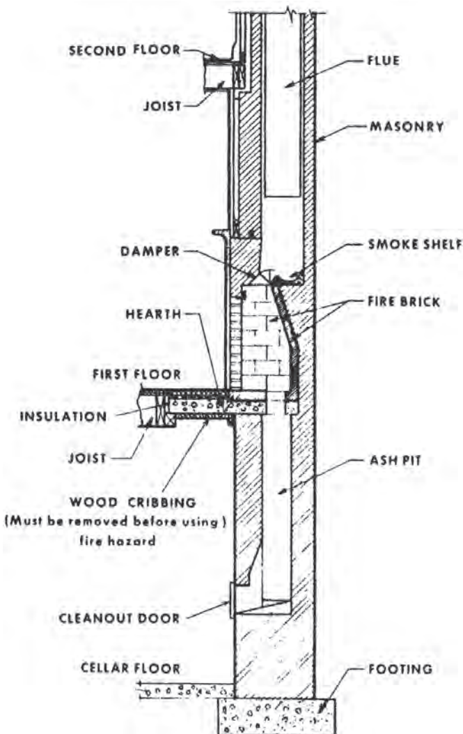
Figure 12.23. Fireplace Construction [4]
