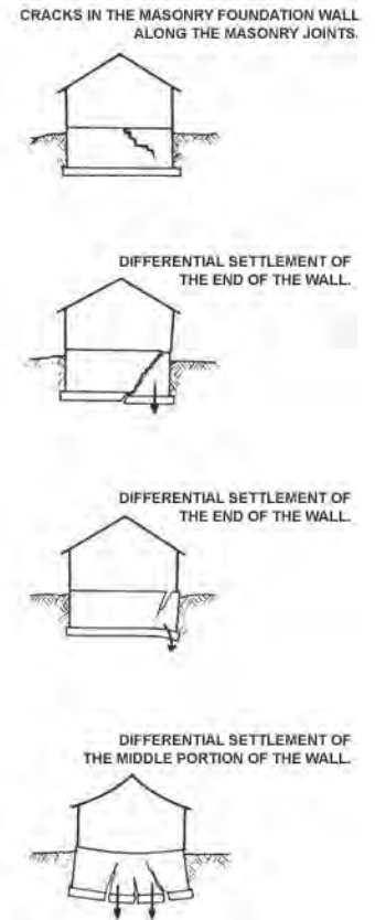
Figure 6.4. Foundation Cracks [4]
