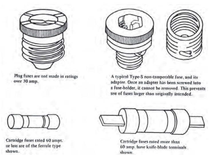
Figure 11.18. Types of Fuses
