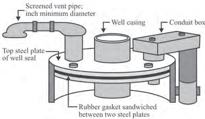
Figure 8.3. Well Seal
