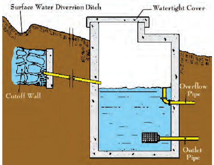
Figure 8.10. Spring Box [5]
