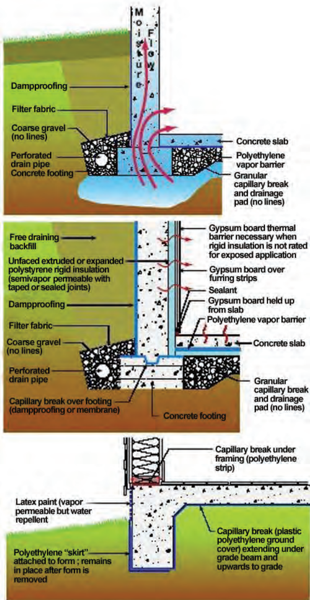
Figure 6.3. Foundation [3]
