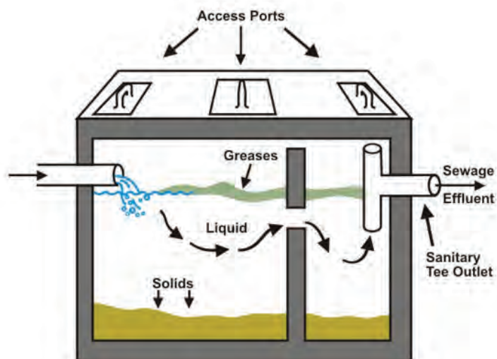
Figure 10.5. Septic Tank [9]
