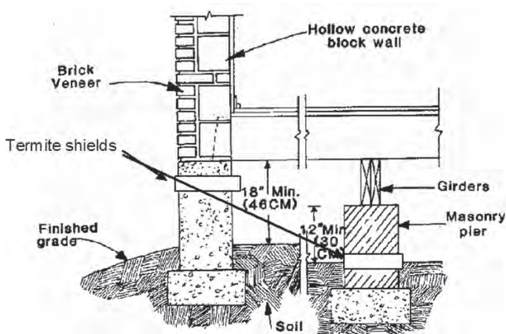
Figure 4.24. Construction Techniques That Discourage Termite Attacks: Thin Metal Termite Shield Should Extend 2 Inches Beyond Foundation and 2 Inches Down [2]
