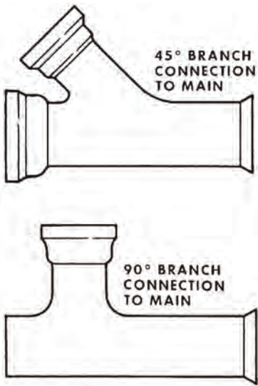
Figure 9.5. Branch Connections
