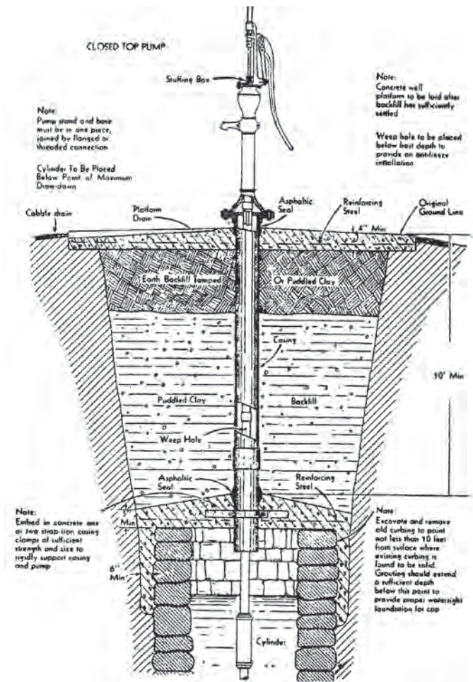
Figure 8.4. Converted Dug Well [1]
