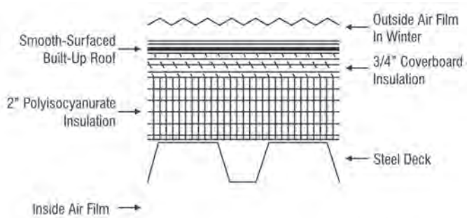
Figure 13.1. Roof Components [2]
