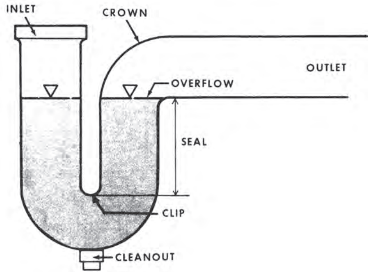
Figure 9.6. P-trap [1]
