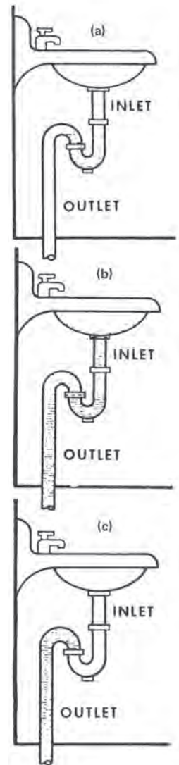
Figure 9.8. Trap Seal: [a] Seal Intact; [b] Fixture Draining; [c] Loss of Gas Seal [1]
