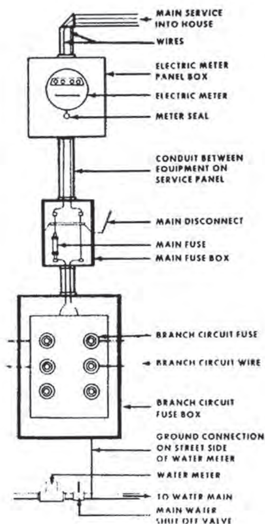
Figure 11.10. Three-wire Service [2]
