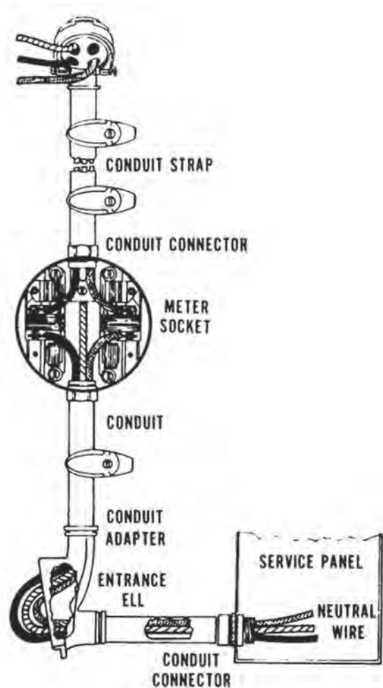
Figure 11.5. Thin-wall Conduit [2]
