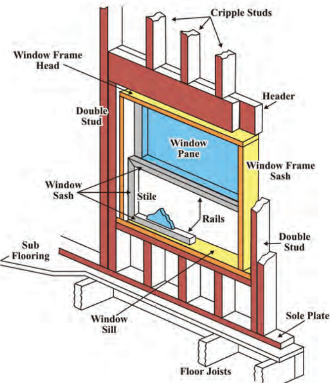
Figure 6.7. Three Dimensional View of a Window [1]
