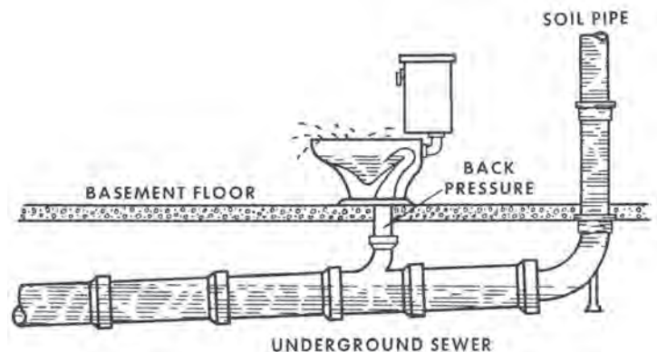
Figure 9.14. Toilet Venting
