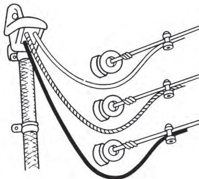
Figure 11.2. Entrance Head
