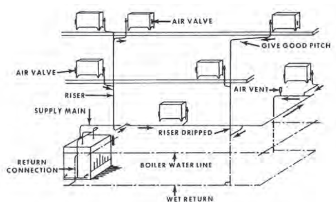
Figure 12.10. Typical Gravity One-pipe Heating System [4]
