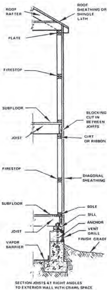
Figure 6.9. Wall Framing [4]
