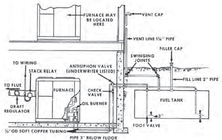
Figure 12.3. Piping Hookup for Buried Outside Tank [4]
