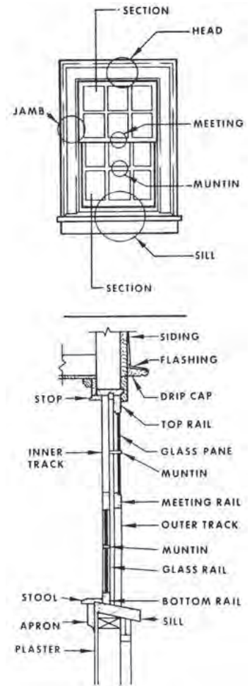
Figure 6.8. Window Details [3]
