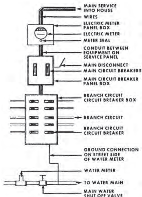
Figure 11.11. Two-wire Service [2]
