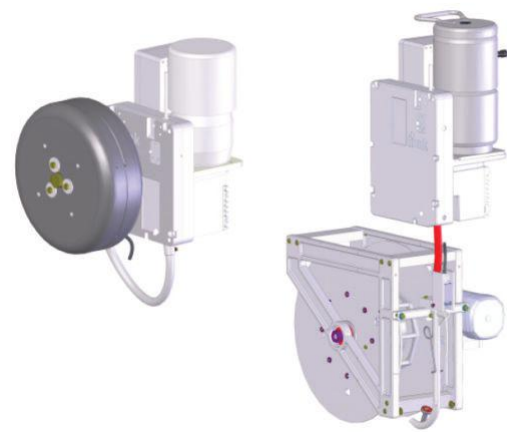
free-running cable reel
