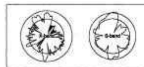
Fig. 7. RCS plot of the Radar Flag (draped) with 0^\circ heel.
