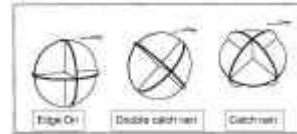
Figure 2. From left to right: An octahedral reflector edge-on to the radar, the double catch-rain position and the catch-rain position.
