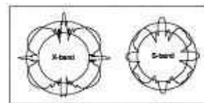
Fig. 4. RCS plot of the Davis Echomaster in the double catch rain position with 0° heel.
