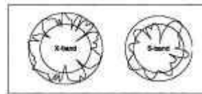
Fig. 6. RCS plot of the Firdell Blipper 210-5 with 0^\circ heel.
