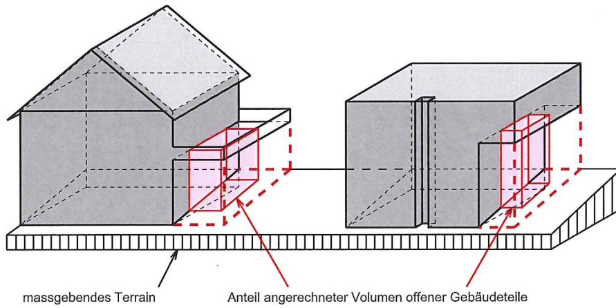
Figur 8.3 Baumassenziffer
