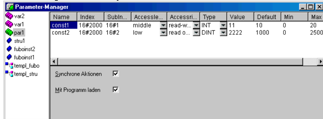
Parameter Manager Editor in CoDeSys
