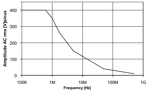
Typical voltage derating PMM511A Measurement category I
