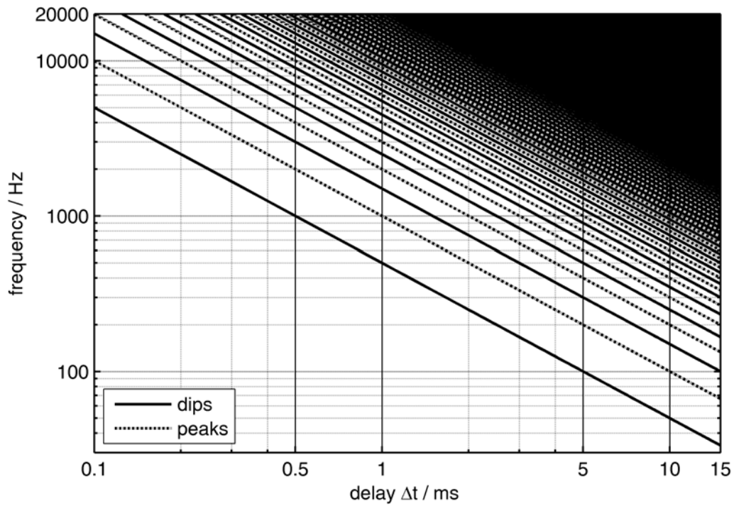
Fig. 2: Position of peaks and dips in a comb-filter-shaped transfer function for different delay times \Delta t
