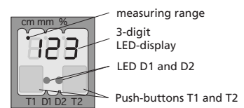
Fig. 3: TouchControl
