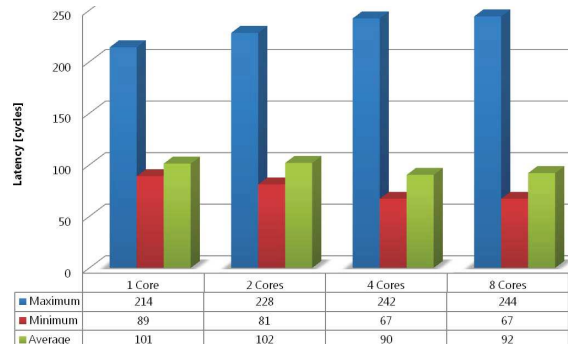
Fig. 2: Write memory access latencies in Freescale P4080
