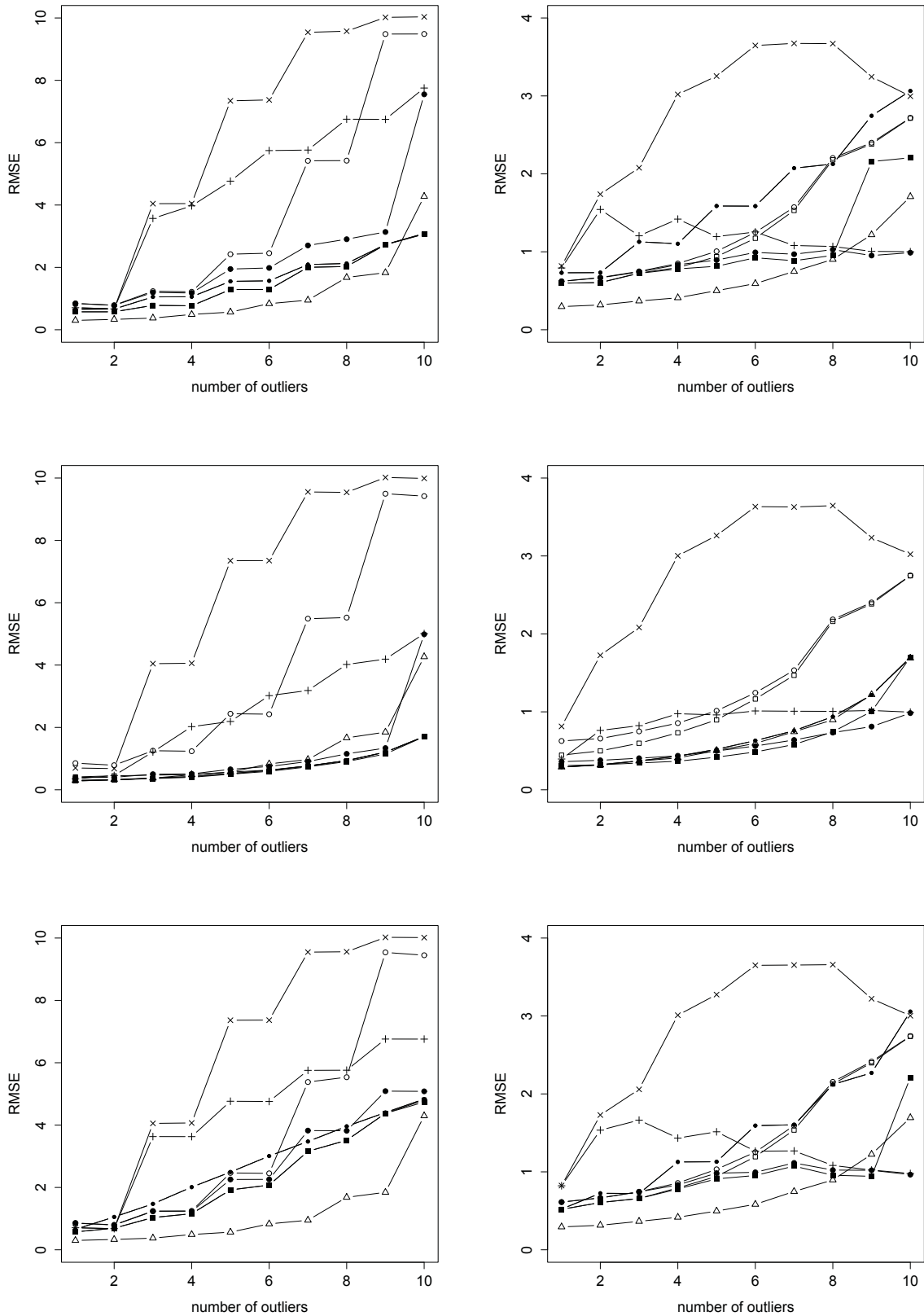
Figure 5: RMSE for positive outlier patches lagged by a half (left) and a full window width, slope \beta = 0.5 (top), \beta = 0.0 (center) and \beta = -0.5 (bottom): median ( \cdot ), RM ( \triangle ), PFMH ( \times ), CFMH ( + ), PRMH ( \circ ), CRMH ( \bullet ), PRMMH ( \square ) and CRMMH ( \blacksquare ).
