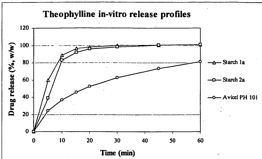
Figure1. In-vitro drug release profiles of pellets containing Starch 1a, Starch 2a, and Avicel PH 101.
