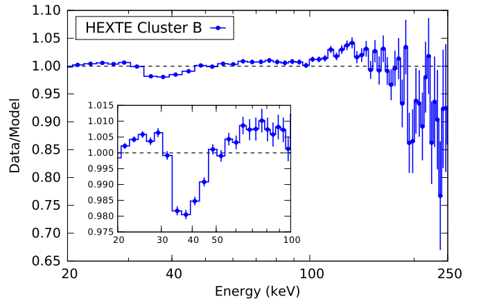
Figure 3. Ratio spectrum for Cluster B created by combining the residual spectra produced by fitting individually our complete sample of 230 selected Crab spectra.
