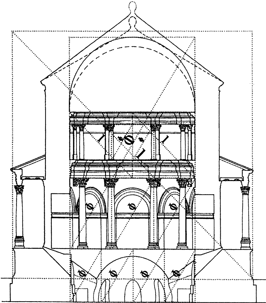
2. Cross-section of Diocletian's mausoleum with proportional scheme. \Phi stands for the golden section ratio ( \frac{\sqrt{5}+1}{2} = 1.61803 ). The dotted line marks the contour of the dome and the roof according to the conjectural (abandoned) original version of the design.
