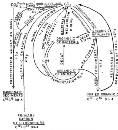
FIGURE 1. The carbon cycle (quantities as cm^3 \times year^{-1} ).
