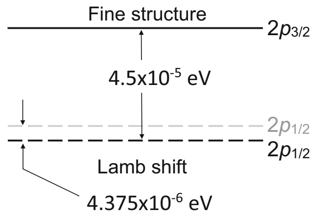
Fig. 1. Energy level diagram for the n = 2 state of the hydrogen atom with the corresponding Lamb shift and fine structure.
