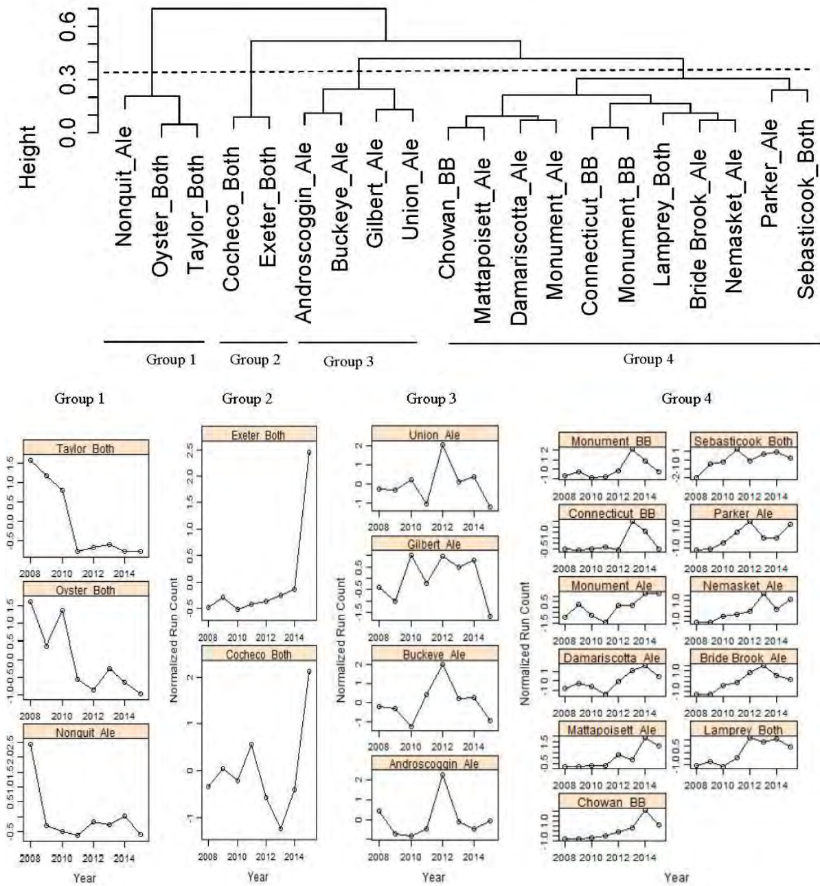
Figure 10. From ASMFC 2017a. Plots of river counts for each grouping associated with the cluster analysis of data from 2008-2015.
