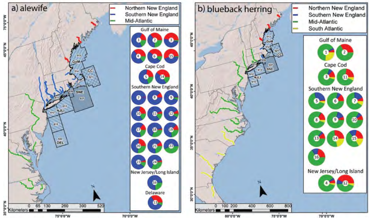
Figure 18. From Hasselman et al. 2016. Relative proportion of assignments to genetic stocks for each bycatch stratum for (a) alewife and (b) blueback herring. The map shows the baseline populations color-coded to coincide with their genetic stock designations and the NOAA statistical areas where bycatch was sampled (grouped by region using various degrees of shading). Pie charts illustrate the relative proportion of bycatch for each stratum, grouped by region that was assigned to each genetic stock.
