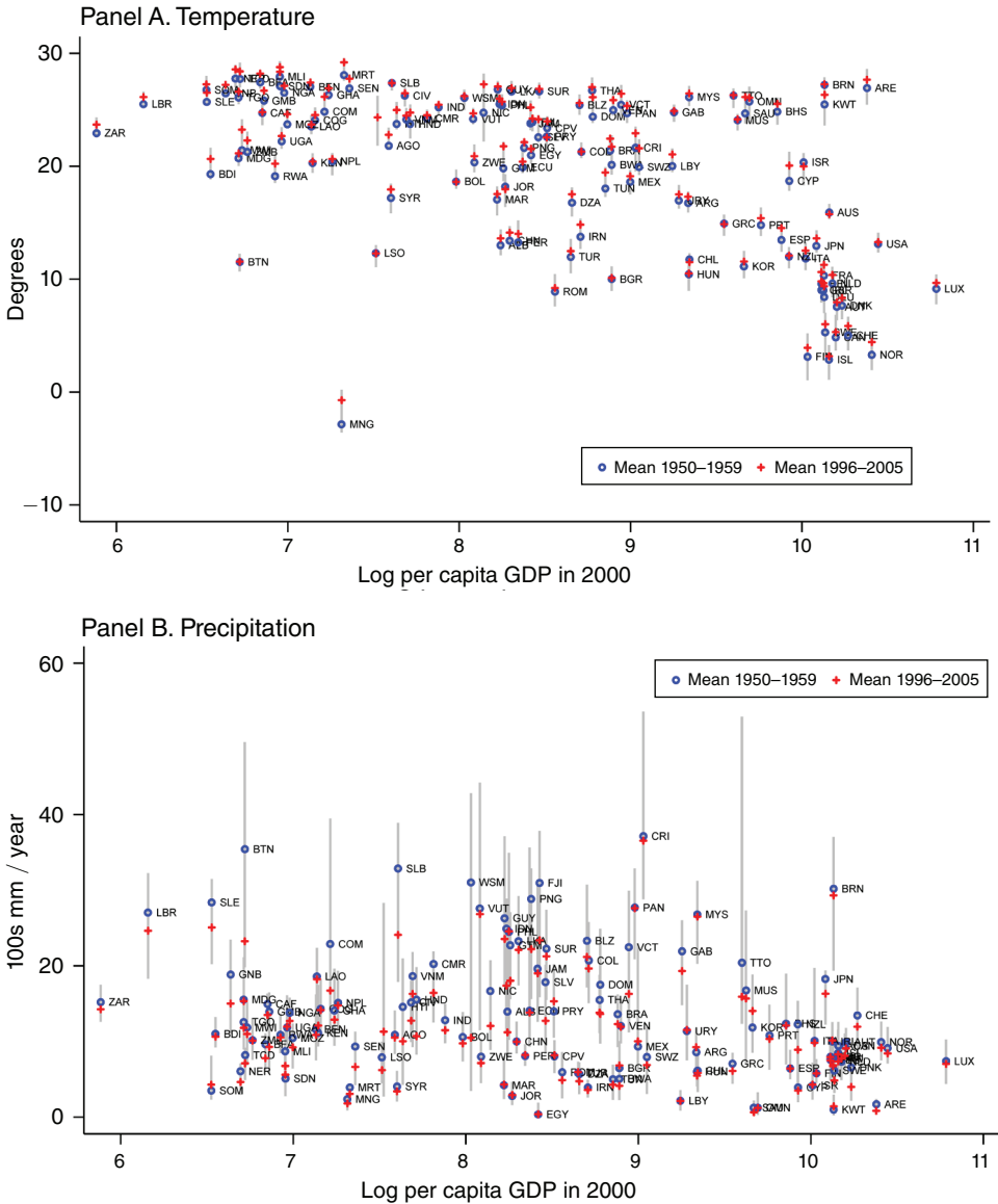
FIGURE 1. CHANGES AND VARIABILITY IN TEMPERATURE AND PRECIPITATION
