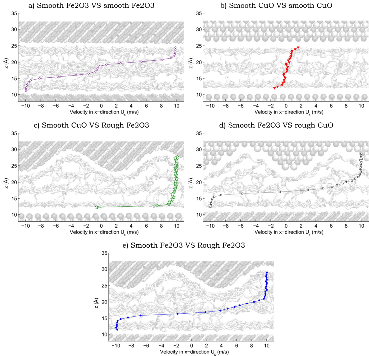
Figure V-14: Velocity profiles across the film thickness for different combinations of wall materials and nano-roughness ( \bar{n}_{\text{CHx}}=0.550 \text{ \AA}^{-2} ).
