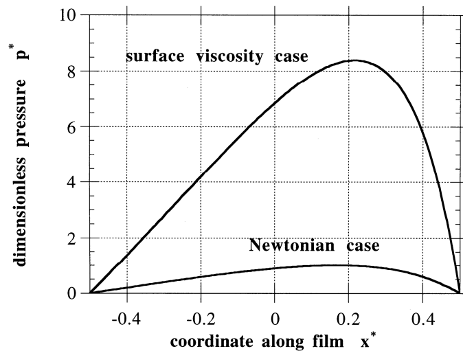
Figure I-22: Pressure generation in a wedge contact with or without the viscosity increase in proximity of surfaces due to the wall-fluid interactions. Results from Sham and Tichy [122].
