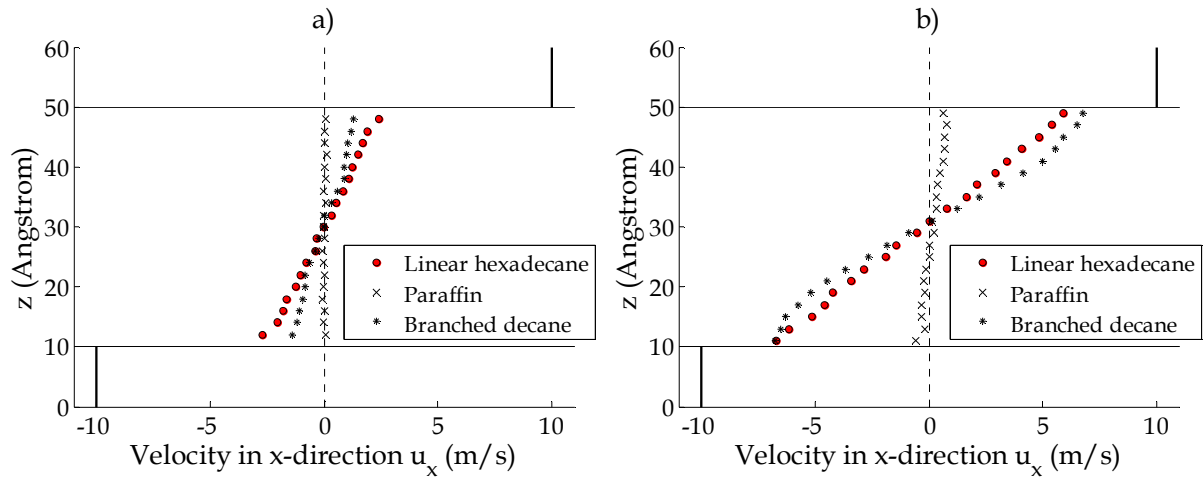
Figure B-4: Velocity profiles for hexadecane, paraffin and 5-Ethyl-2-methyldecane confined between canonical surfaces. a) Cubic structure with lattice constant a=3 \text{ \AA} ; b) Face-Centered-Cubic structure with lattice constant a=4.5 \text{ \AA} . P=0.5 \text{ GPa} , u_2=-u_1=10 \text{ m/s} , h=4 \text{ nm} , T_{\text{wall}}=300\text{K} .
