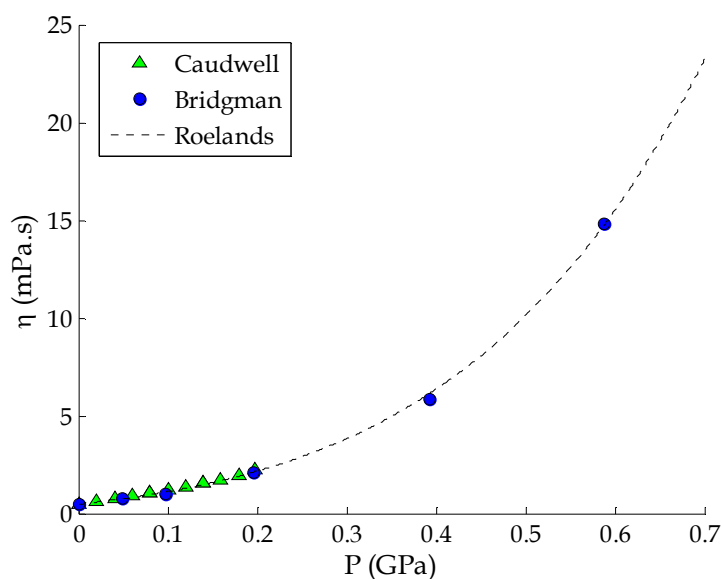
Figure IV-6: Roelands viscosity-pressure dependence for n-octane, from results by [154, 155].
