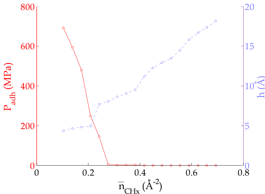
Figure V-5: Normal adhesion pressure and film thickness as a function of the quantity of n-hexadecane in the contact. Smooth Fe_2O_3 walls, P=0.5 GPa, u_2=-u_1=10 m/s, T_{wall}=300K .
