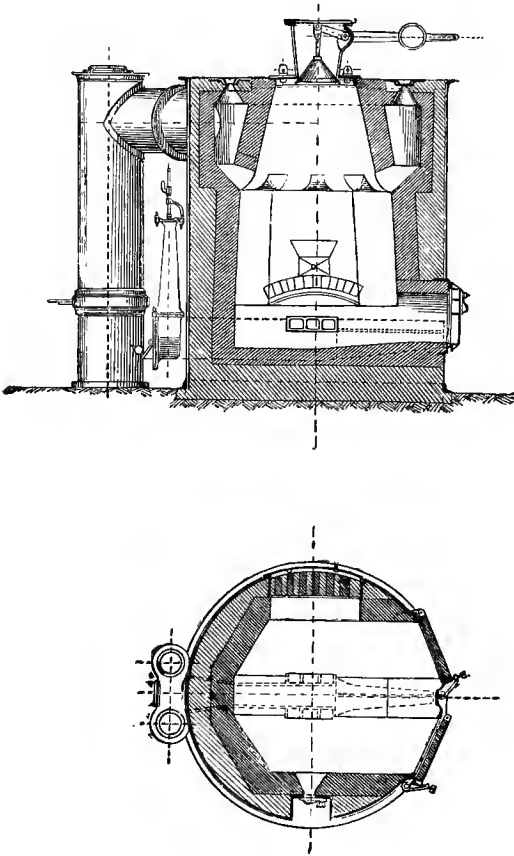
FIG. 55.—THE WILSON GAS PRODUCER.
