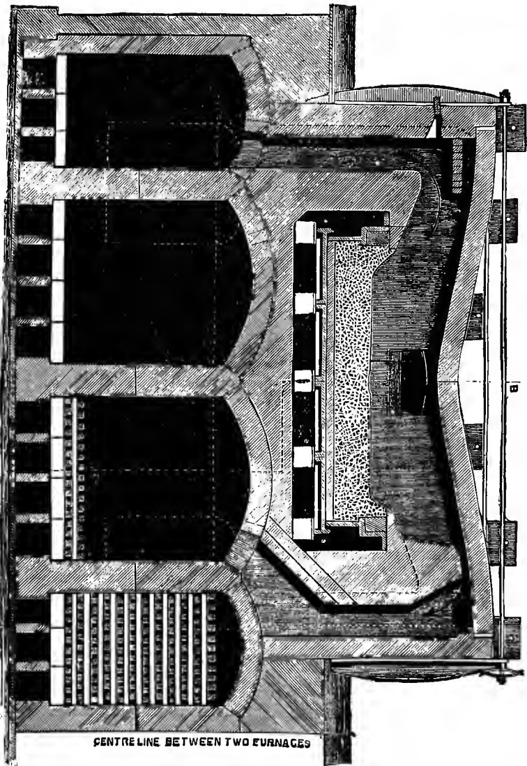
FIG. 56.—SIEMENS' REGENERATOR.
