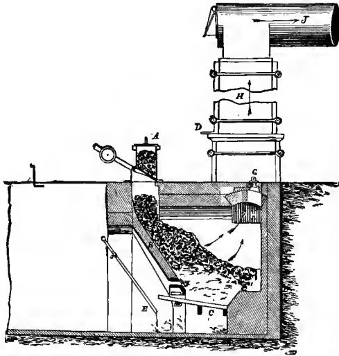
FIG. 54.—SIEMENS' GAS PRODUCER.
