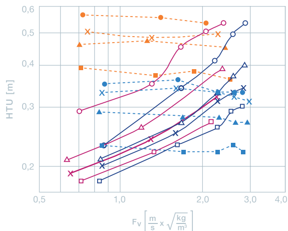
HTU: VFF-Twin-Pak® No. 2 vs. Pall-50-M
