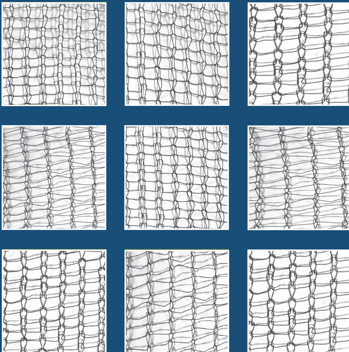
Examples of different droplet separator wire meshes.
