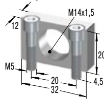
MB14SC2-V4A Montageblock
