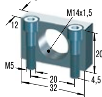
MB14SC2 Montageblock
