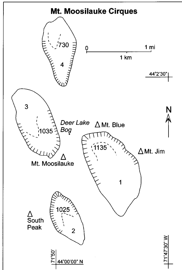
FIGURE 4. Cirque morphometric map for Mount Moosilauke. Solid lines indicate outlines of cirques, hachured solid lines are cirque headwalls, dashed lines are cirque schrunds, with altitudes indicated in meters. Numbers refer to Table I.
