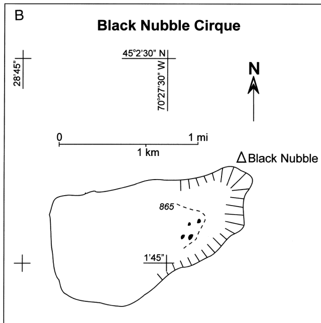
FIGURE 6. A. Cirque morphometric maps for Longfellow Mountains, Maine. Solid lines indicate outlines of cirques, hachured solid lines are cirque headwalls, dashed lines are cirque schrunds, with altitudes indicated in meters. Numbers for cirques on Sugarloaf and Crocker Mountains refer to Table I; only cirque #6 has small water body, shown in black. B. Black Nubble cirque; water bodies shown in black.
