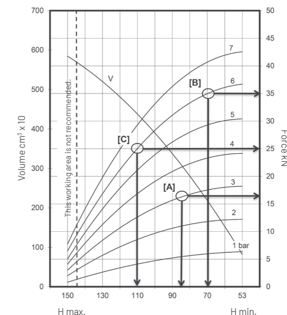
Aerolator F-1B-310 data chart Datendiagramm Aerolator F-1B-310
