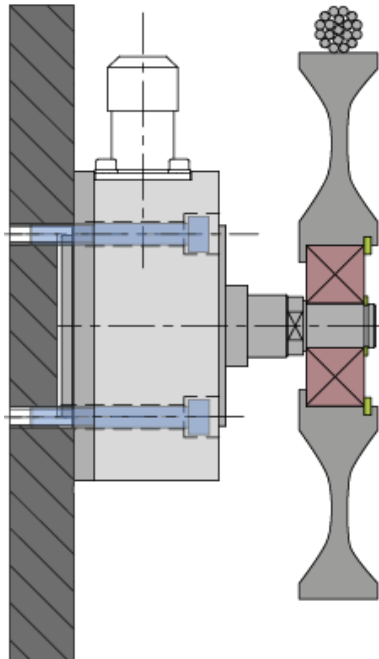
Figure 3: Pilot mount
