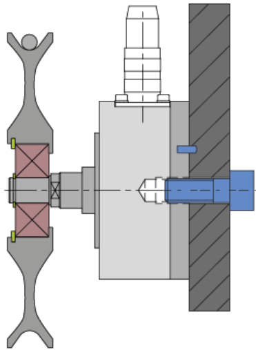
Figure 5: Flat mount
