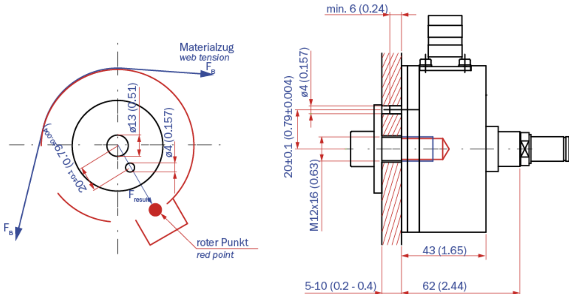
Figure 6: dimension machine frame for FL mount
