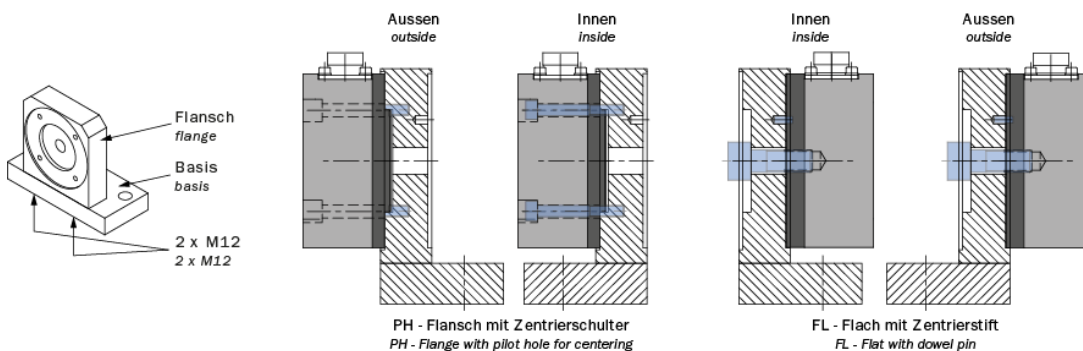
Figure 7: installation bracket CA203.MB
