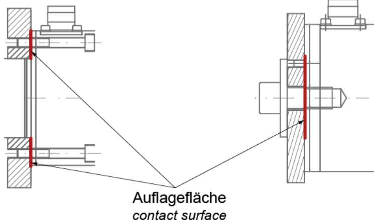
Figure 2: contact surface
