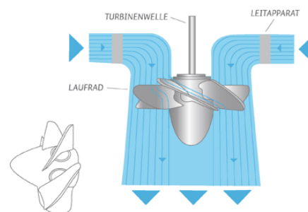
Kaplan-Turbine
