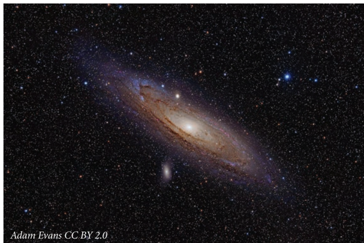
The Andromeda Galaxy
